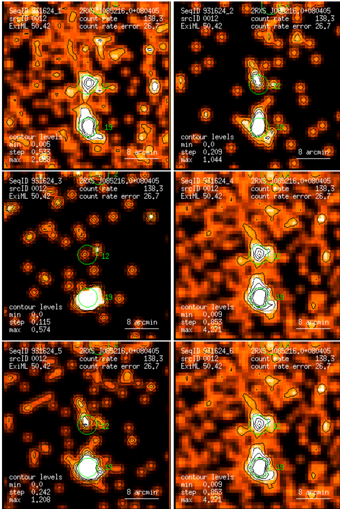
Figure 12: RASS 931624: detection 0012: band rate images, Gaussian filter: (1) PSPC channels 11 – 41, (2) 52 – 90, (3) 91 – 201, (4) 11 – 235, (5) 52 – 201, (6) 11 – 201. Broad band rates in counts/ks. Band rate contour levels in counts/ks/arcmin 2 .
