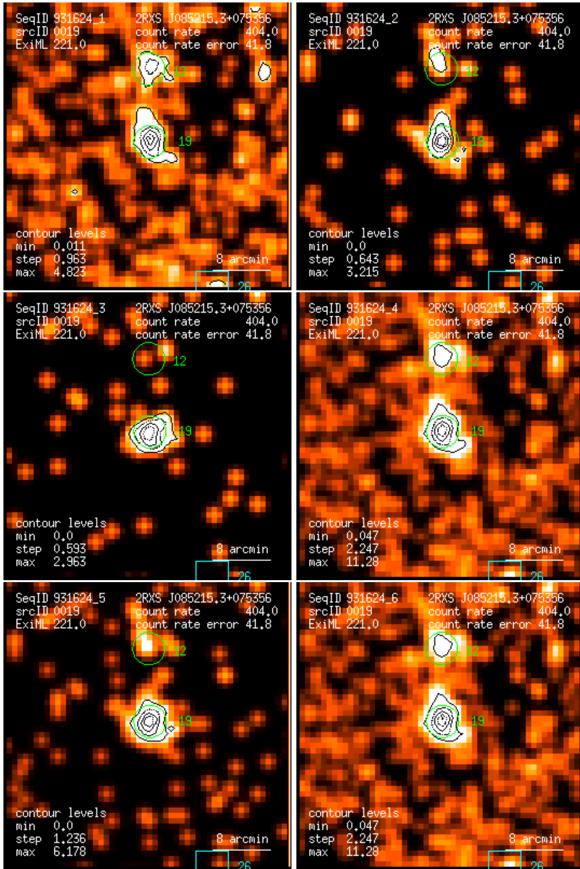
Figure 19: RASS 931624: detection 0019: band rate images, Gaussian filter: (1) PSPC channels 11 – 41, (2) 52 – 90, (3) 91 – 201, (4) 11 – 235, (5) 52 – 201, (6) 11 – 201. Broad band rates in counts/ks. Band rate contour levels in counts/ks/arcmin 2 .
