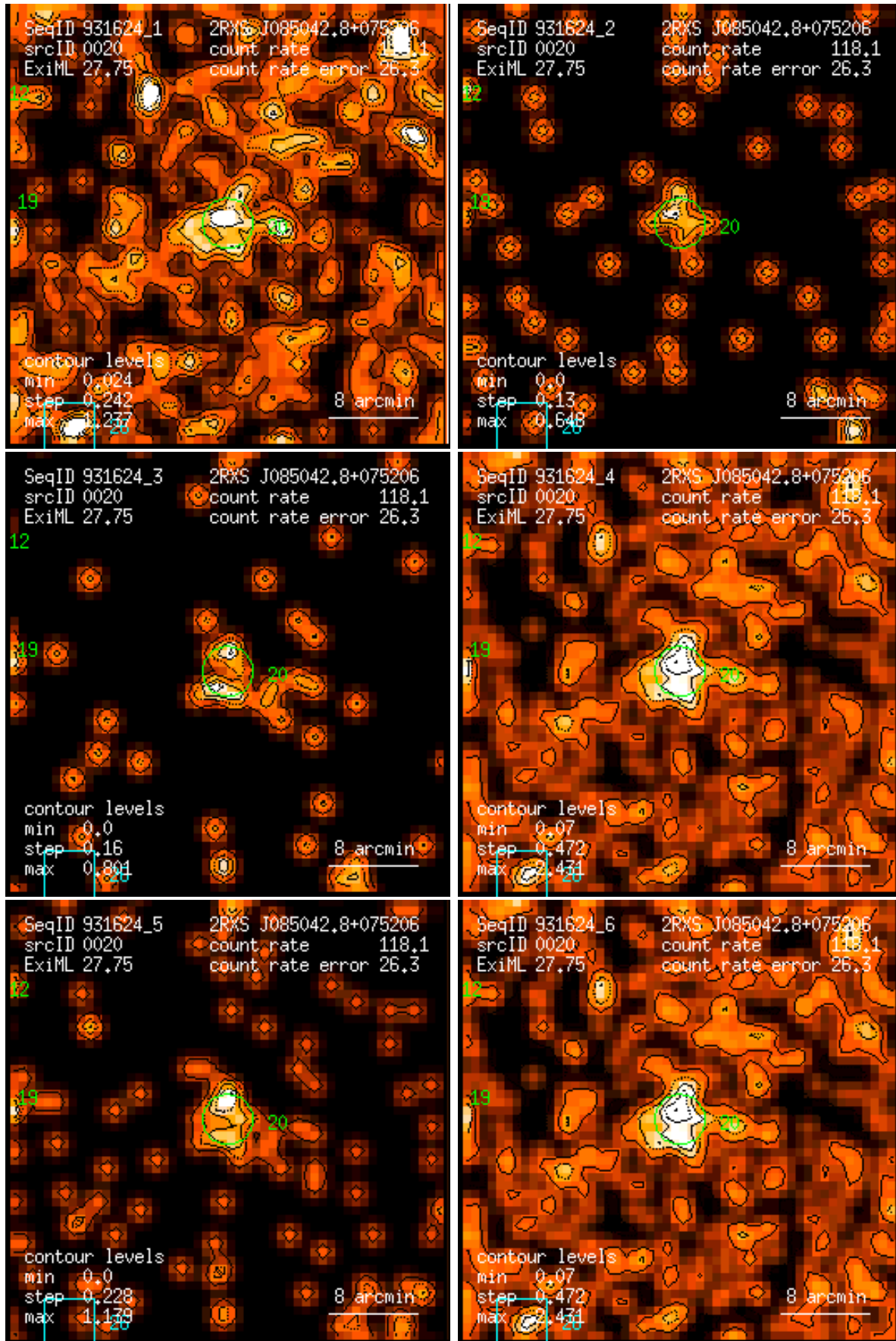
Figure 20: RASS 931624: detection 0020: band rate images, Gaussian filter: (1) PSPC channels 11 – 41, (2) 52 – 90, (3) 91 – 201, (4) 11 – 235, (5) 52 – 201, (6) 11 – 201. Broad band rates in counts/ks. Band rate contour levels in counts/ks/arcmin 2 .
