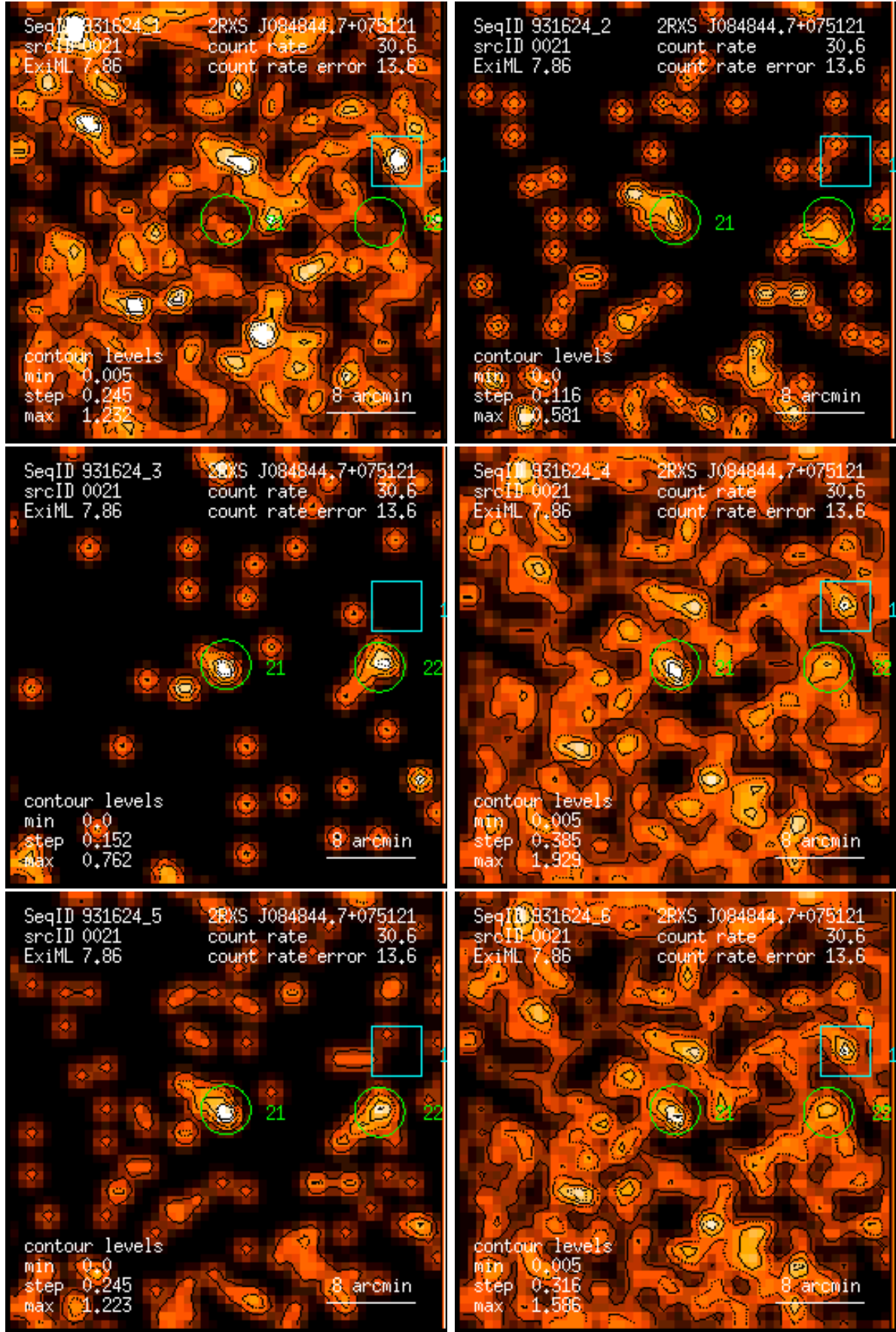
Figure 21: RASS 931624: detection 0021: band rate images, Gaussian filter: (1) PSPC channels 11 – 41, (2) 52 – 90, (3) 91 – 201, (4) 11 – 235, (5) 52 – 201, (6) 11 – 201. Broad band rates in counts/ks. Band rate contour levels in counts/ks/arcmin 2 .
