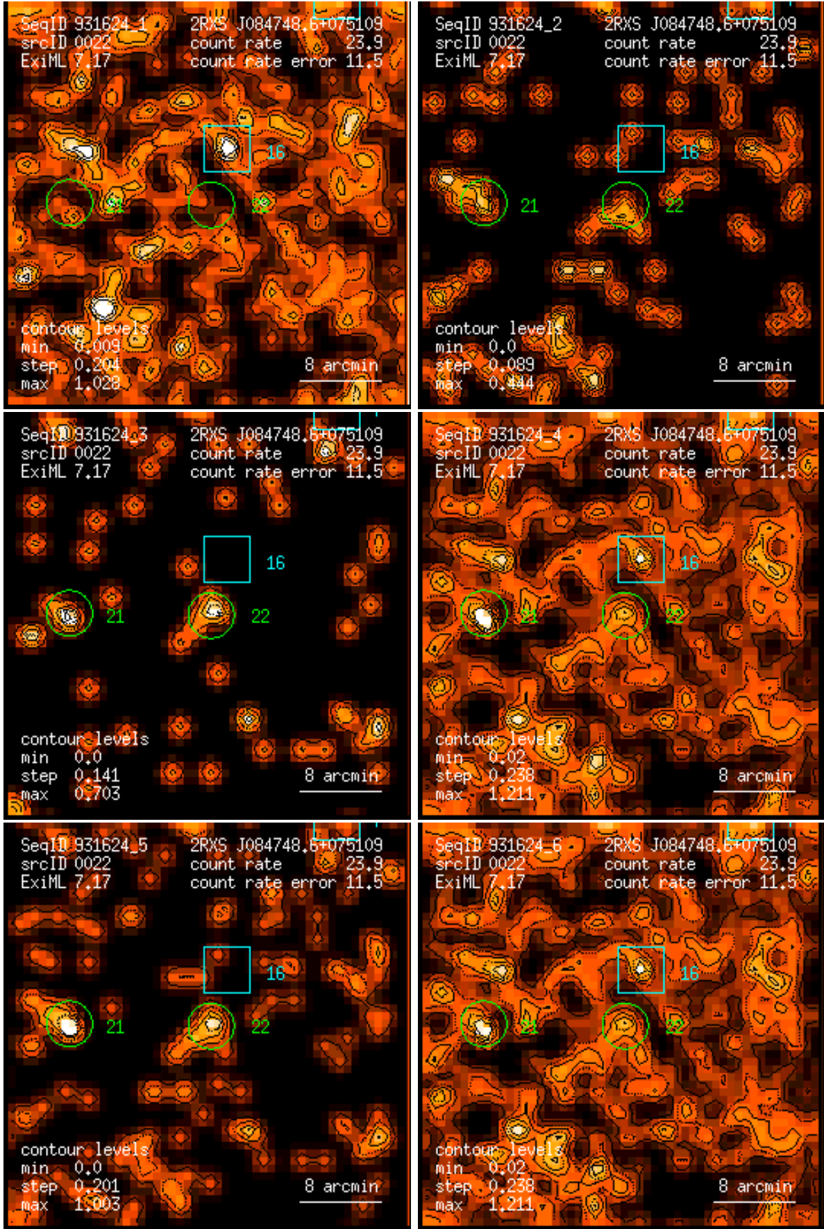
Figure 22: RASS 931624: detection 0022: band rate images, Gaussian filter: (1) PSPC channels 11 – 41, (2) 52 – 90, (3) 91 – 201, (4) 11 – 235, (5) 52 – 201, (6) 11 – 201. Broad band rates in counts/ks. Band rate contour levels in counts/ks/arcmin 2 .
