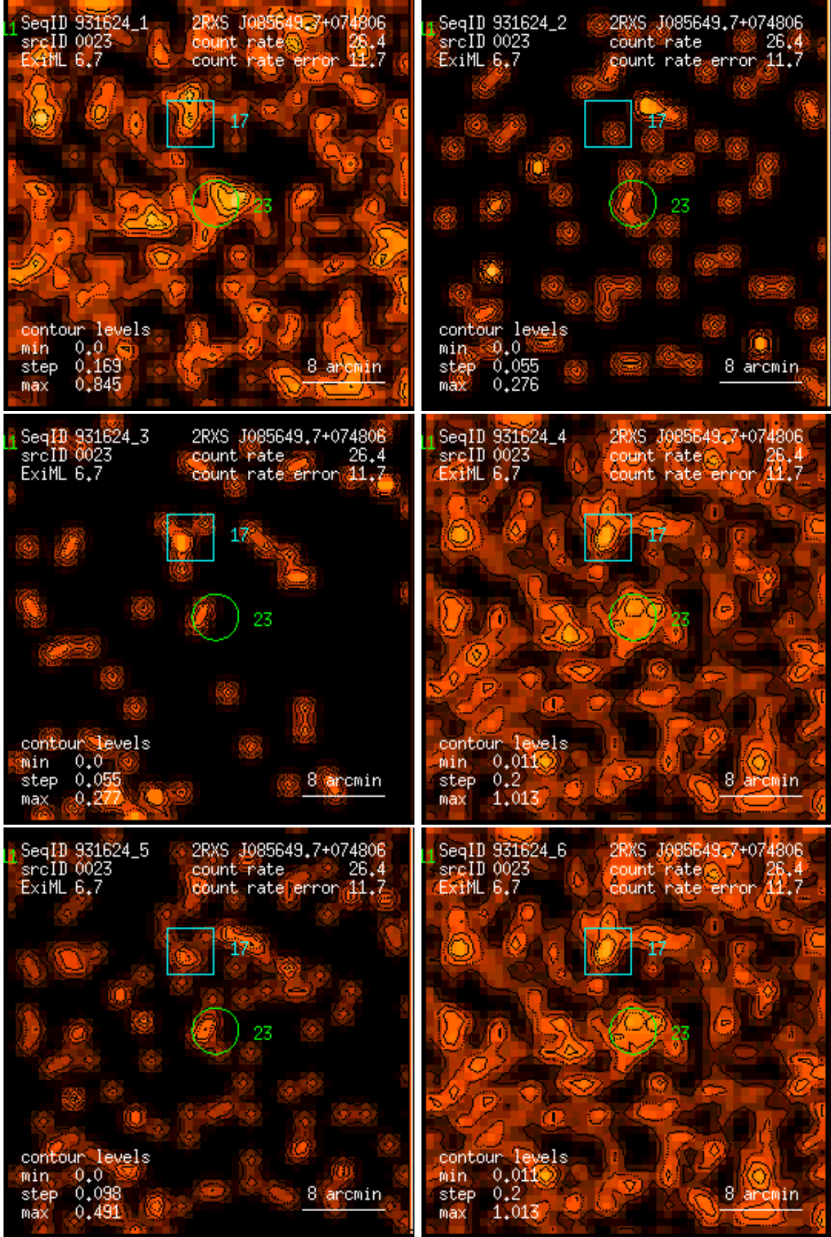
Figure 23: RASS 931624: detection 0023: band rate images, Gaussian filter: (1) PSPC channels 11 – 41, (2) 52 – 90, (3) 91 – 201, (4) 11 – 235, (5) 52 – 201, (6) 11 – 201. Broad band rates in counts/ks. Band rate contour levels in counts/ks/arcmin 2 .
