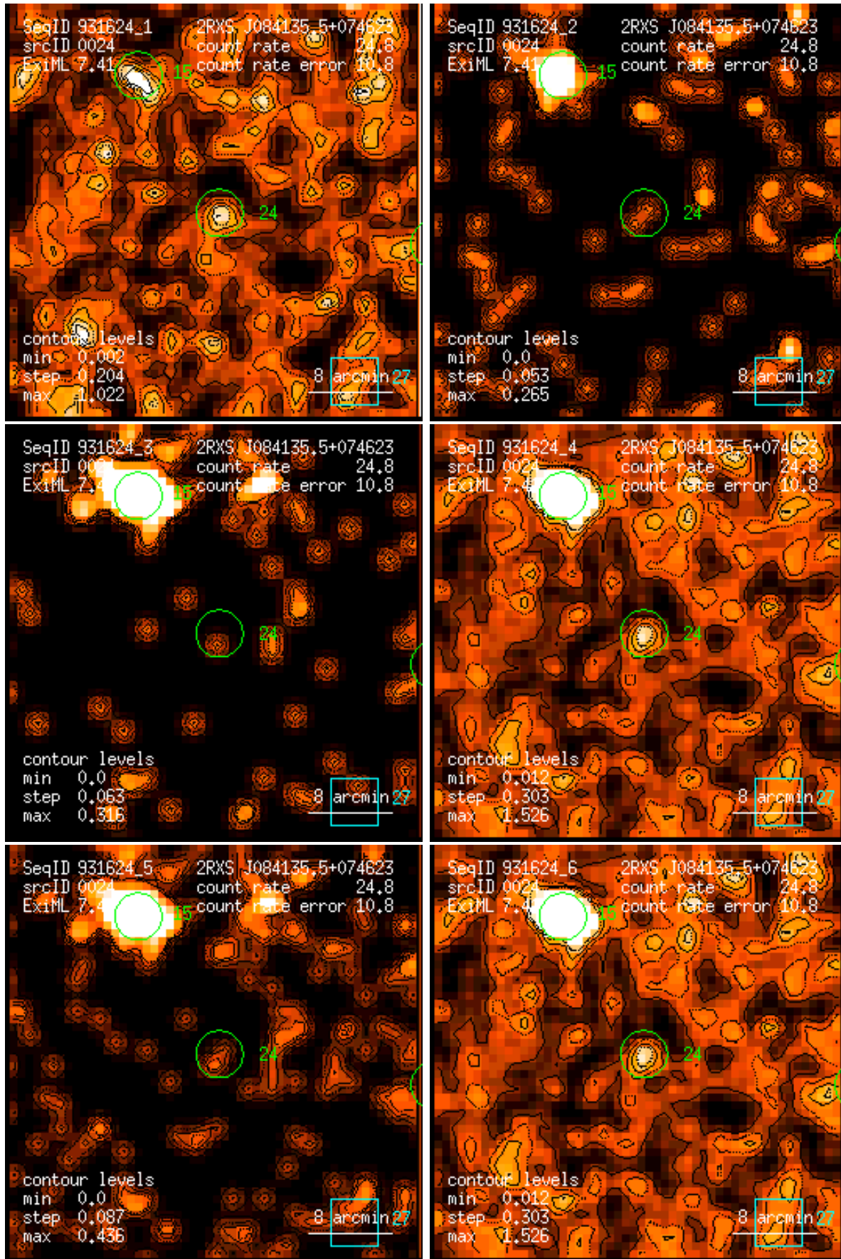
Figure 24: RASS 931624: detection 0024: band rate images, Gaussian filter: (1) PSPC channels 11 – 41, (2) 52 – 90, (3) 91 – 201, (4) 11 – 235, (5) 52 – 201, (6) 11 – 201. Broad band rates in counts/ks. Band rate contour levels in counts/ks/arcmin 2 .
