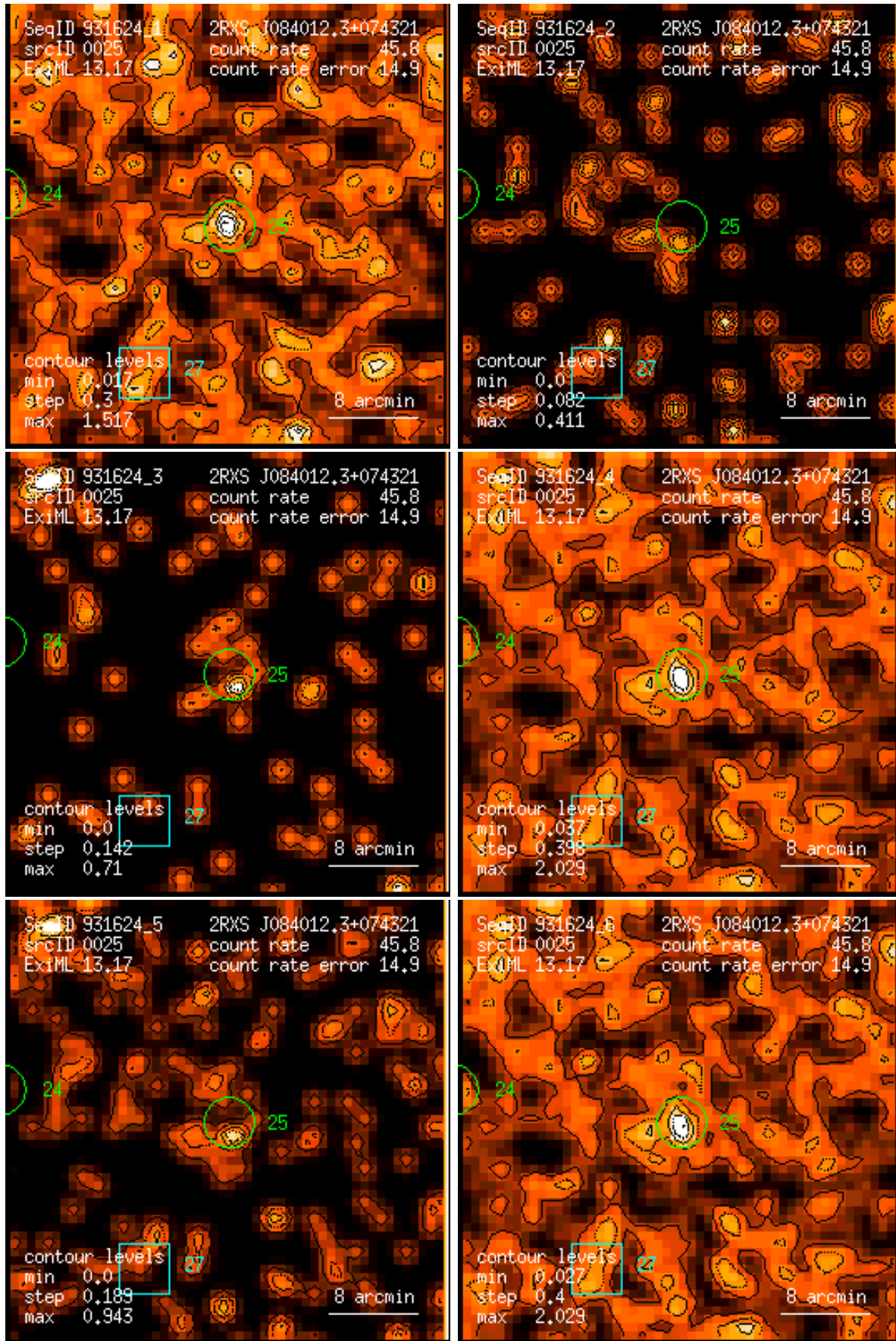
Figure 25: RASS 931624: detection 0025: band rate images, Gaussian filter: (1) PSPC channels 11 – 41, (2) 52 – 90, (3) 91 – 201, (4) 11 – 235, (5) 52 – 201, (6) 11 – 201. Broad band rates in counts/ks. Band rate contour levels in counts/ks/arcmin 2 .
