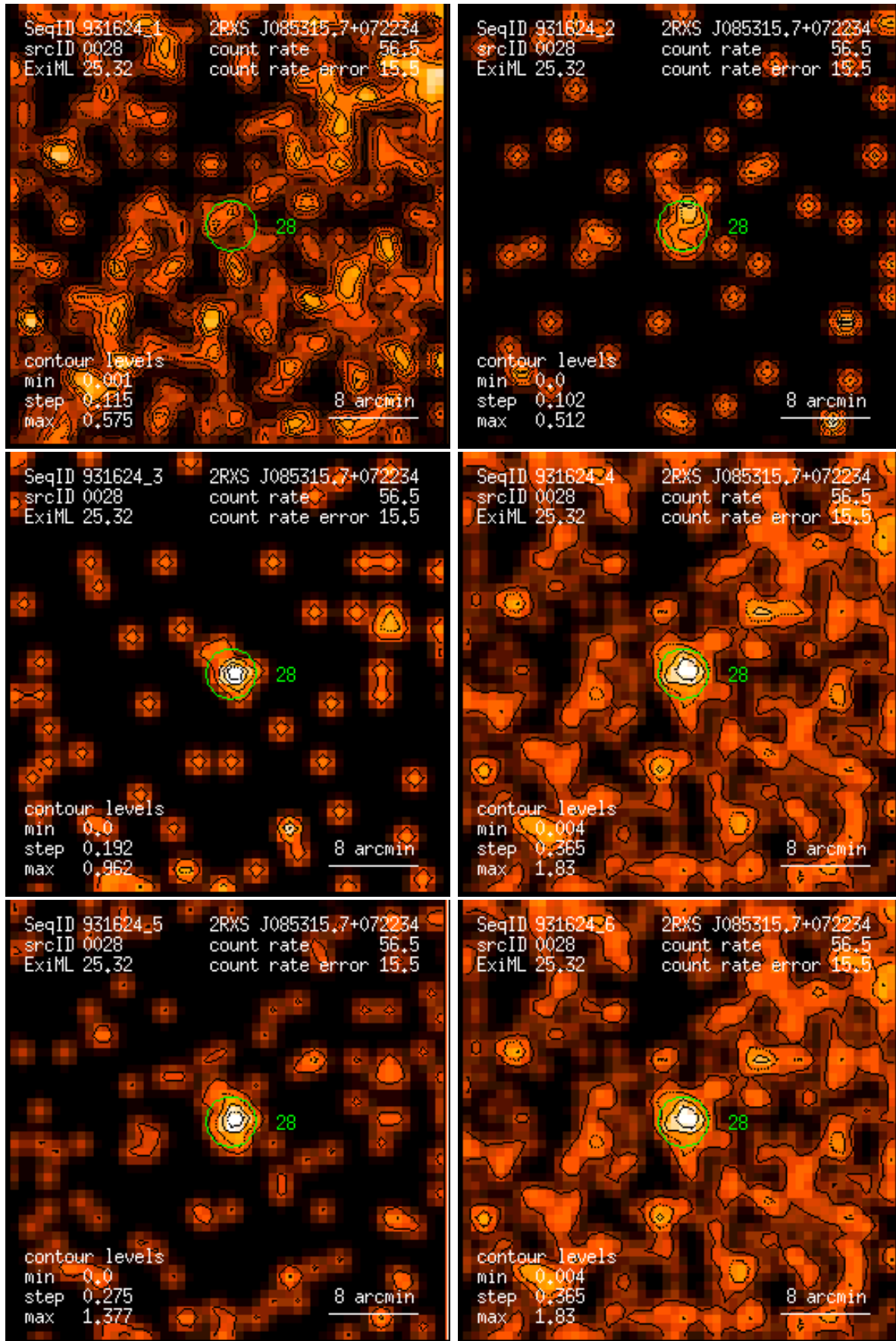
Figure 28: RASS 931624: detection 0028: band rate images, Gaussian filter: (1) PSPC channels 11 – 41, (2) 52 – 90, (3) 91 – 201, (4) 11 – 235, (5) 52 – 201, (6) 11 – 201. Broad band rates in counts/ks. Band rate contour levels in counts/ks/arcmin 2 .
