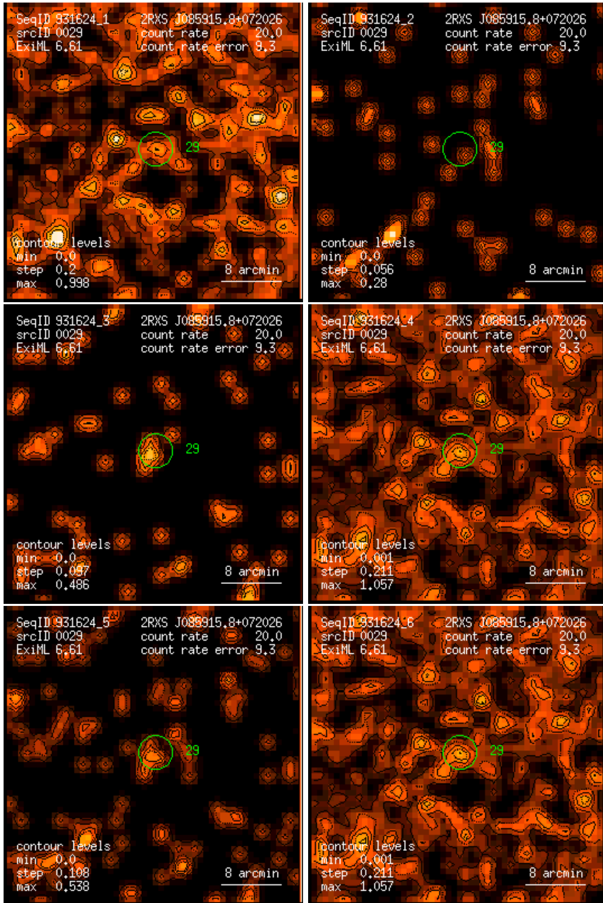
Figure 29: RASS 931624: detection 0029: band rate images, Gaussian filter: (1) PSPC channels 11 – 41, (2) 52 – 90, (3) 91 – 201, (4) 11 – 235, (5) 52 – 201, (6) 11 – 201. Broad band rates in counts/ks. Band rate contour levels in counts/ks/arcmin 2 .
