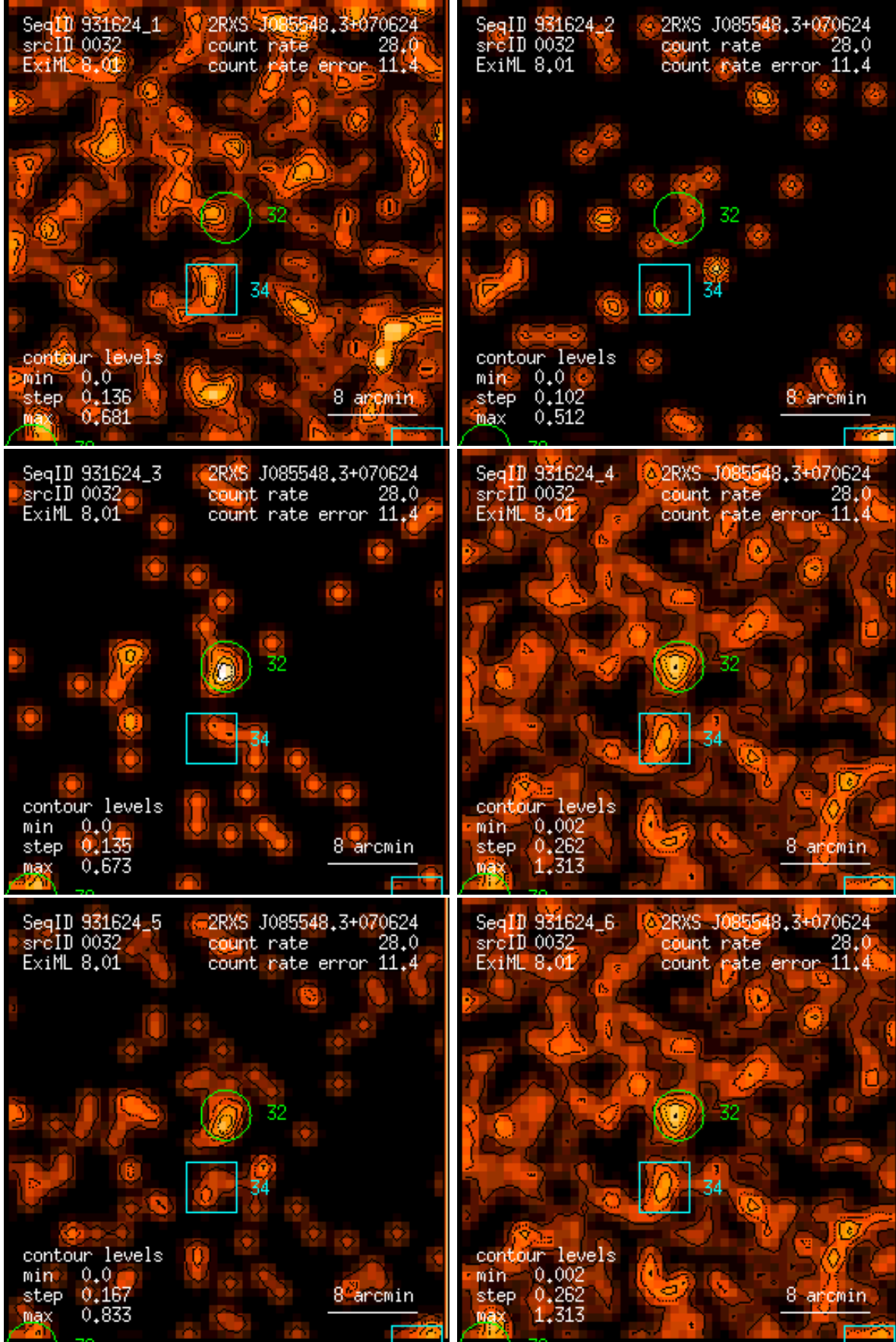
Figure 32: RASS 931624: detection 0032: band rate images, Gaussian filter: (1) PSPC channels 11 – 41, (2) 52 – 90, (3) 91 – 201, (4) 11 – 235, (5) 52 – 201, (6) 11 – 201. Broad band rates in counts/ks. Band rate contour levels in counts/ks/arcmin 2 .
