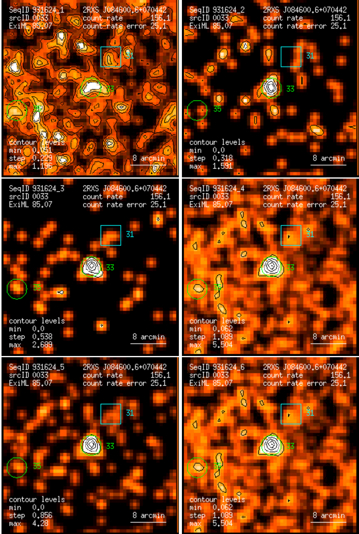
Figure 33: RASS 931624: detection 0033: band rate images, Gaussian filter: (1) PSPC channels 11 – 41, (2) 52 – 90, (3) 91 – 201, (4) 11 – 235, (5) 52 – 201, (6) 11 – 201. Broad band rates in counts/ks. Band rate contour levels in counts/ks/arcmin 2 .
