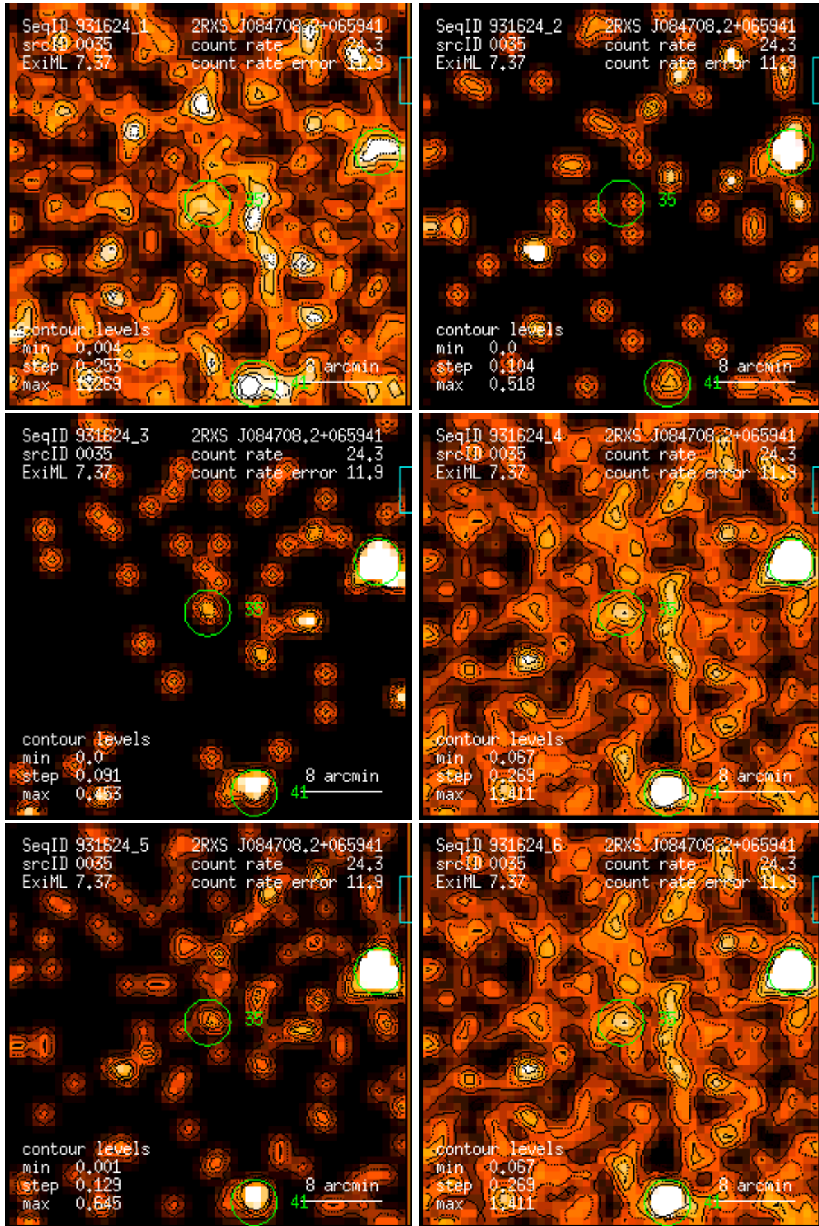
Figure 35: RASS 931624: detection 0035: band rate images, Gaussian filter: (1) PSPC channels 11 – 41, (2) 52 – 90, (3) 91 – 201, (4) 11 – 235, (5) 52 – 201, (6) 11 – 201. Broad band rates in counts/ks. Band rate contour levels in counts/ks/arcmin 2 .
