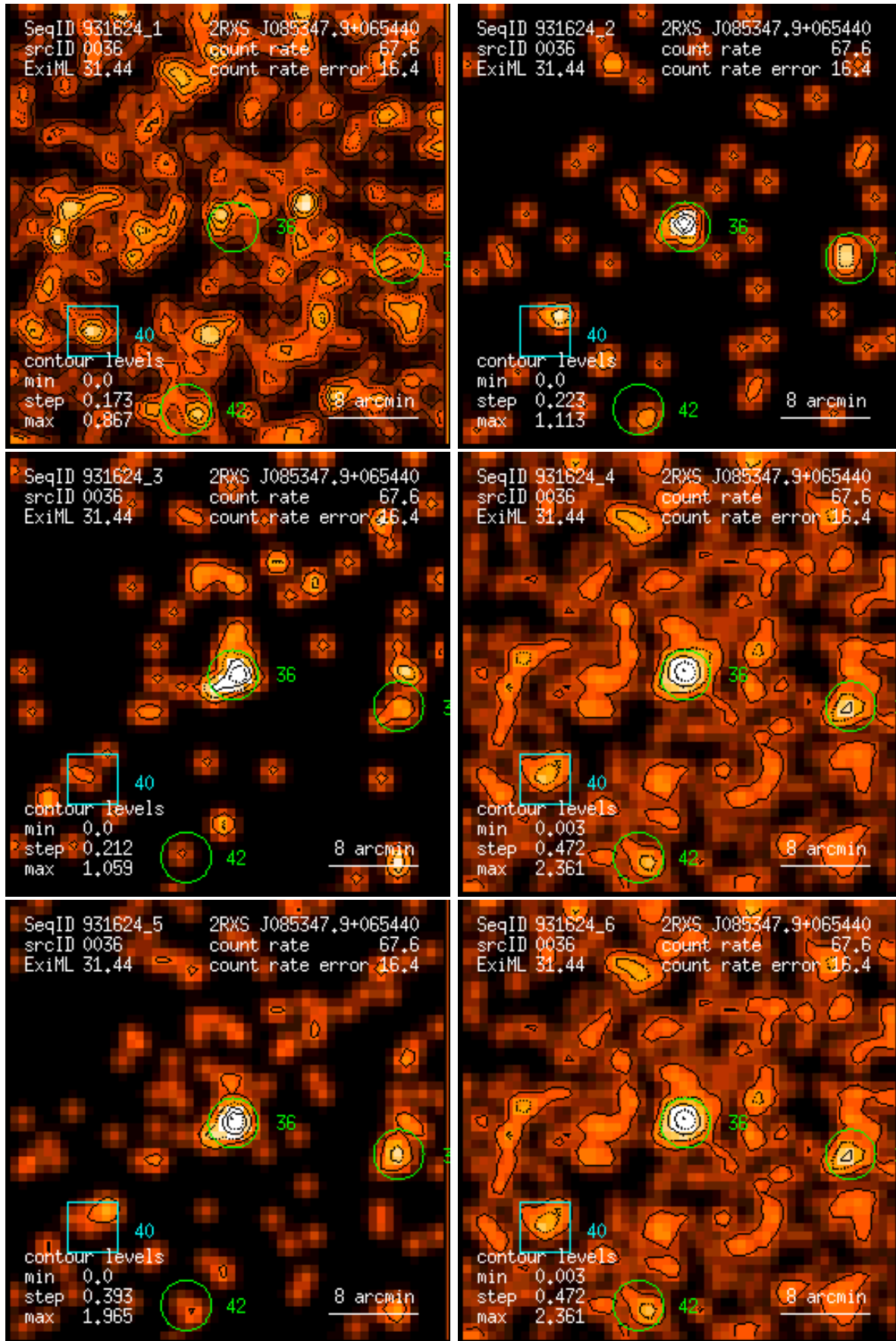
Figure 36: RASS 931624: detection 0036: band rate images, Gaussian filter: (1) PSPC channels 11 – 41, (2) 52 – 90, (3) 91 – 201, (4) 11 – 235, (5) 52 – 201, (6) 11 – 201. Broad band rates in counts/ks. Band rate contour levels in counts/ks/arcmin 2 .
