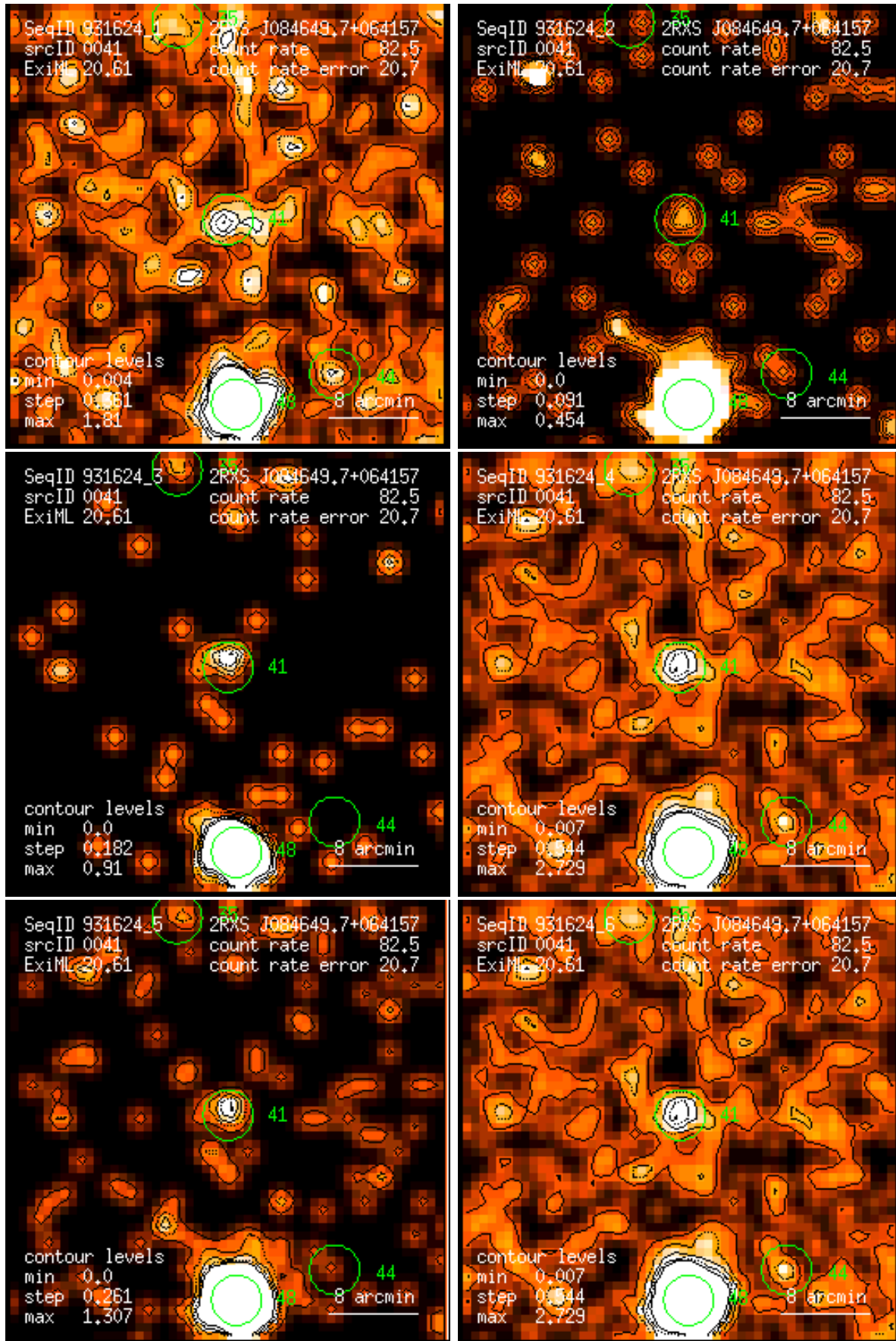
Figure 41: RASS 931624: detection 0041: band rate images, Gaussian filter: (1) PSPC channels 11 – 41, (2) 52 – 90, (3) 91 – 201, (4) 11 – 235, (5) 52 – 201, (6) 11 – 201. Broad band rates in counts/ks. Band rate contour levels in counts/ks/arcmin 2 .
