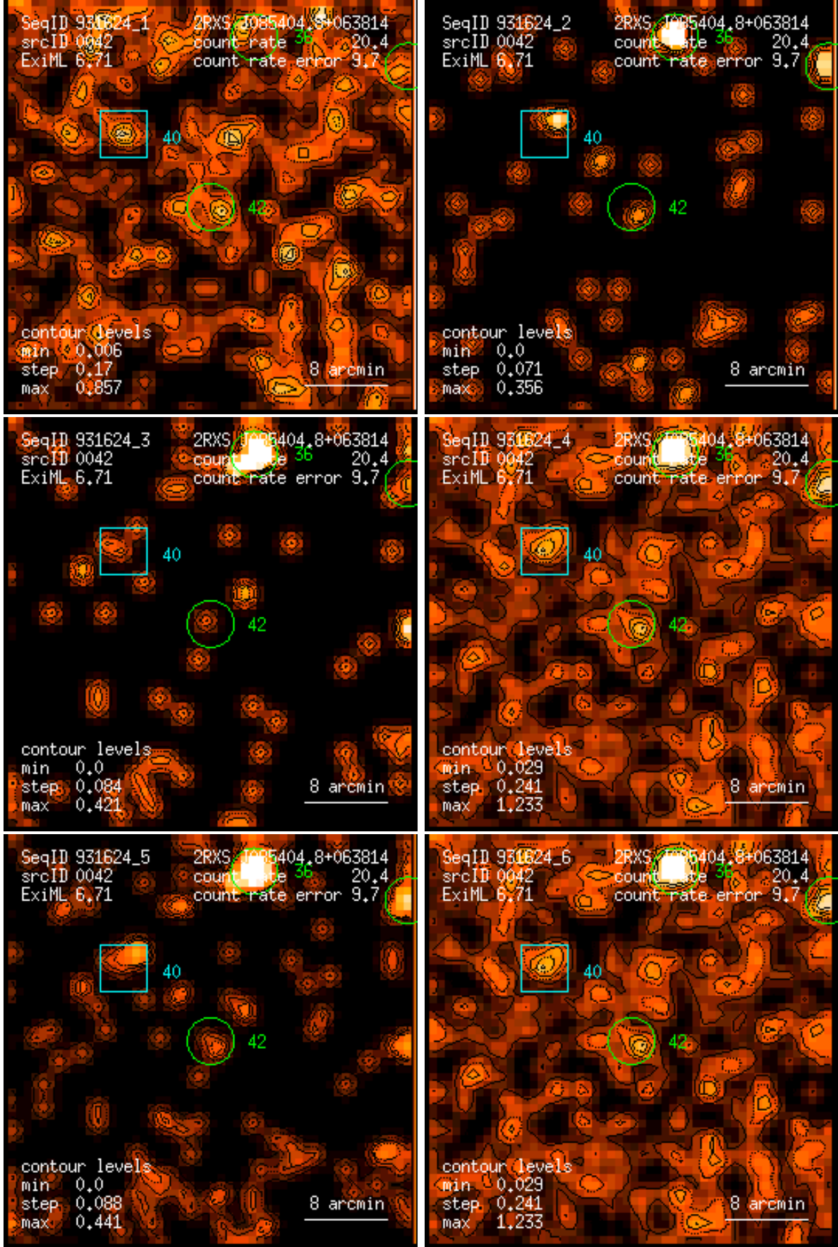
Figure 42: RASS 931624: detection 0042: band rate images, Gaussian filter: (1) PSPC channels 11 – 41, (2) 52 – 90, (3) 91 – 201, (4) 11 – 235, (5) 52 – 201, (6) 11 – 201. Broad band rates in counts/ks. Band rate contour levels in counts/ks/arcmin 2 .
