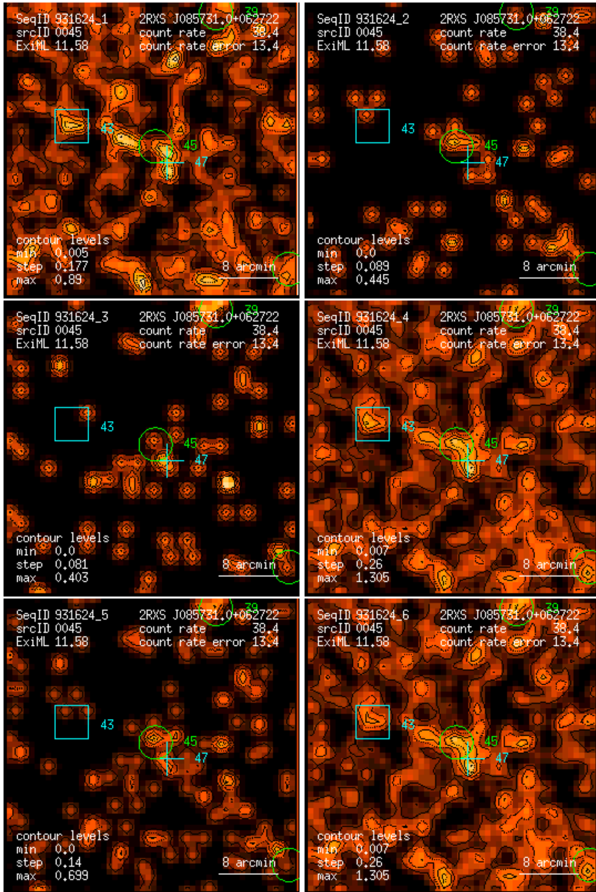
Figure 45: RASS 931624: detection 0045: band rate images, Gaussian filter: (1) PSPC channels 11 – 41, (2) 52 – 90, (3) 91 – 201, (4) 11 – 235, (5) 52 – 201, (6) 11 – 201. Broad band rates in counts/ks. Band rate contour levels in counts/ks/arcmin 2 .
