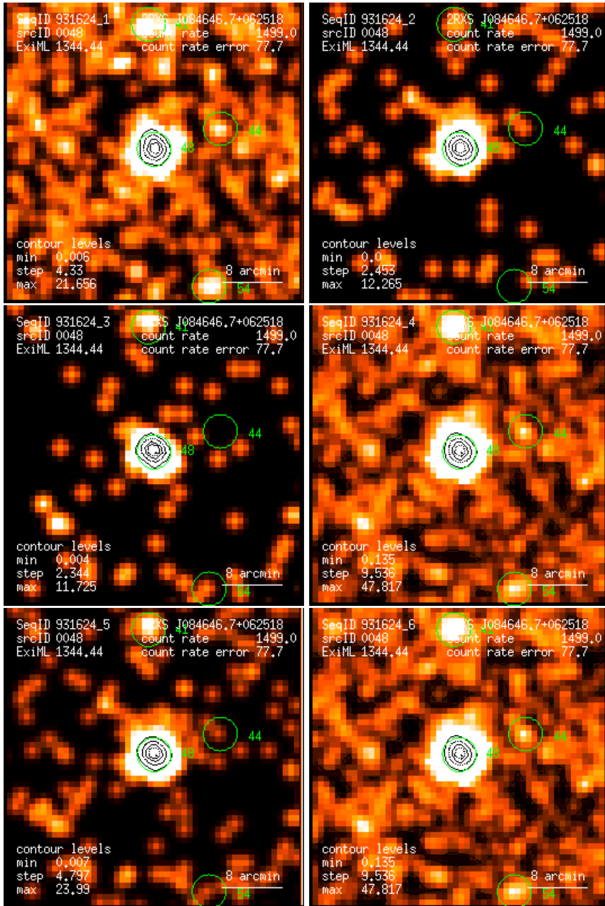
Figure 48: RASS 931624: detection 0048: band rate images, Gaussian filter: (1) PSPC channels 11 – 41, (2) 52 – 90, (3) 91 – 201, (4) 11 – 235, (5) 52 – 201, (6) 11 – 201. Broad band rates in counts/ks. Band rate contour levels in counts/ks/arcmin 2 .
