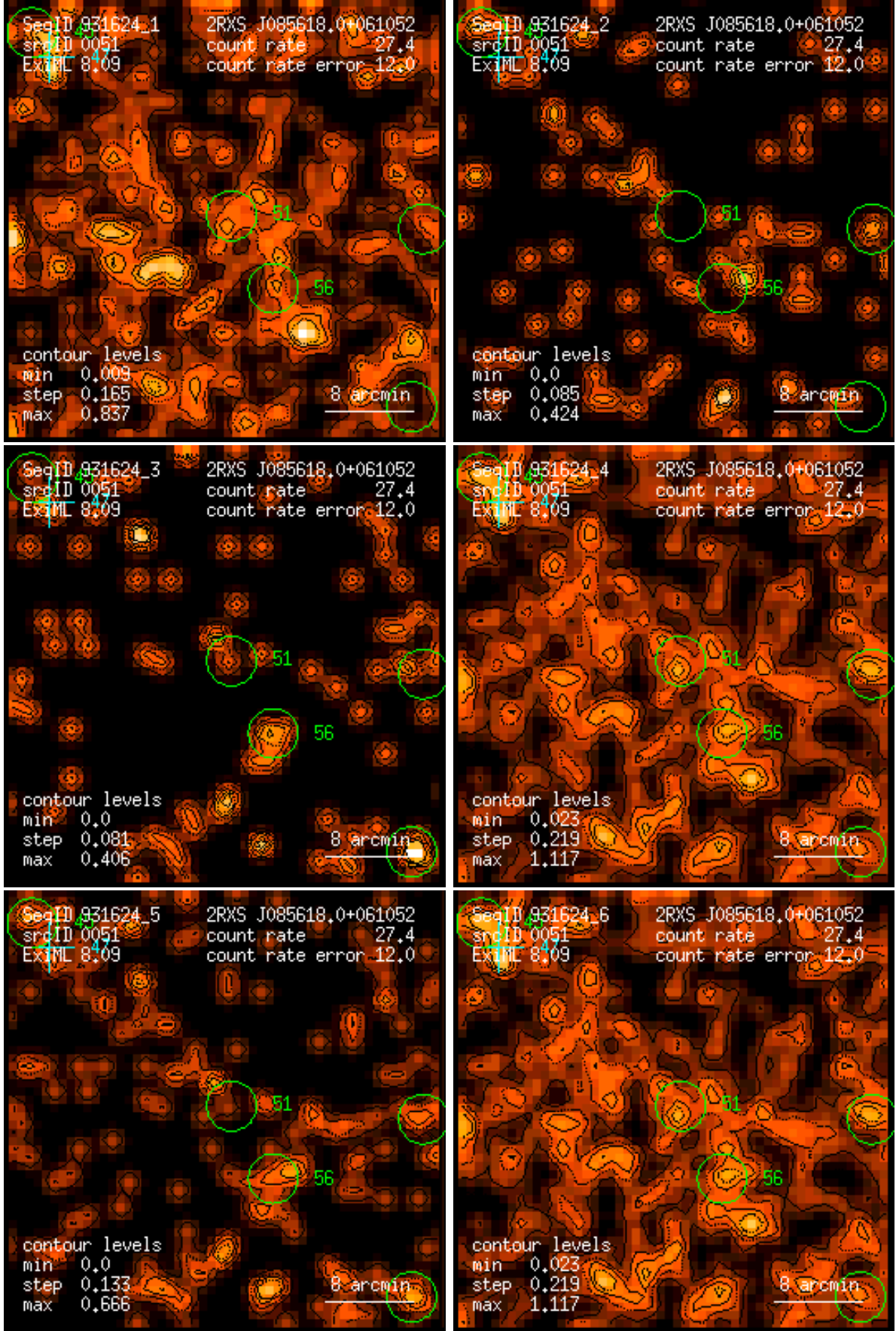
Figure 51: RASS 931624: detection 0051: band rate images, Gaussian filter: (1) PSPC channels 11 – 41, (2) 52 – 90, (3) 91 – 201, (4) 11 – 235, (5) 52 – 201, (6) 11 – 201. Broad band rates in counts/ks. Band rate contour levels in counts/ks/arcmin 2 .
