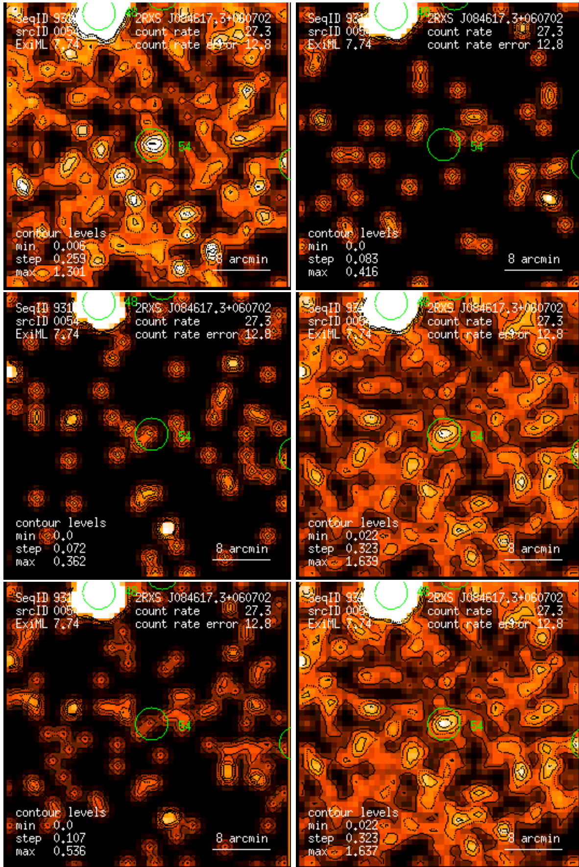
Figure 54: RASS 931624: detection 0054: band rate images, Gaussian filter: (1) PSPC channels 11 – 41, (2) 52 – 90, (3) 91 – 201, (4) 11 – 235, (5) 52 – 201, (6) 11 – 201. Broad band rates in counts/ks. Band rate contour levels in counts/ks/arcmin 2 .
