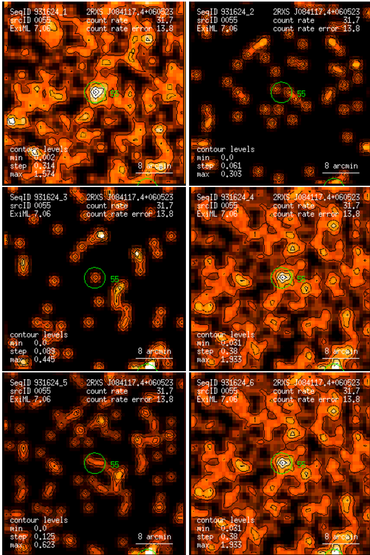
Figure 55: RASS 931624: detection 0055: band rate images, Gaussian filter: (1) PSPC channels 11 – 41, (2) 52 – 90, (3) 91 – 201, (4) 11 – 235, (5) 52 – 201, (6) 11 – 201. Broad band rates in counts/ks. Band rate contour levels in counts/ks/arcmin 2 .
