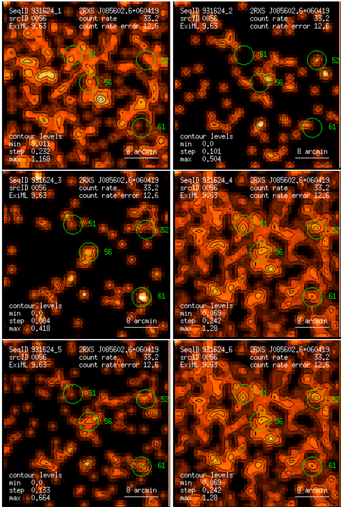
Figure 56: RASS 931624: detection 0056: band rate images, Gaussian filter: (1) PSPC channels 11 – 41, (2) 52 – 90, (3) 91 – 201, (4) 11 – 235, (5) 52 – 201, (6) 11 – 201. Broad band rates in counts/ks. Band rate contour levels in counts/ks/arcmin 2 .
