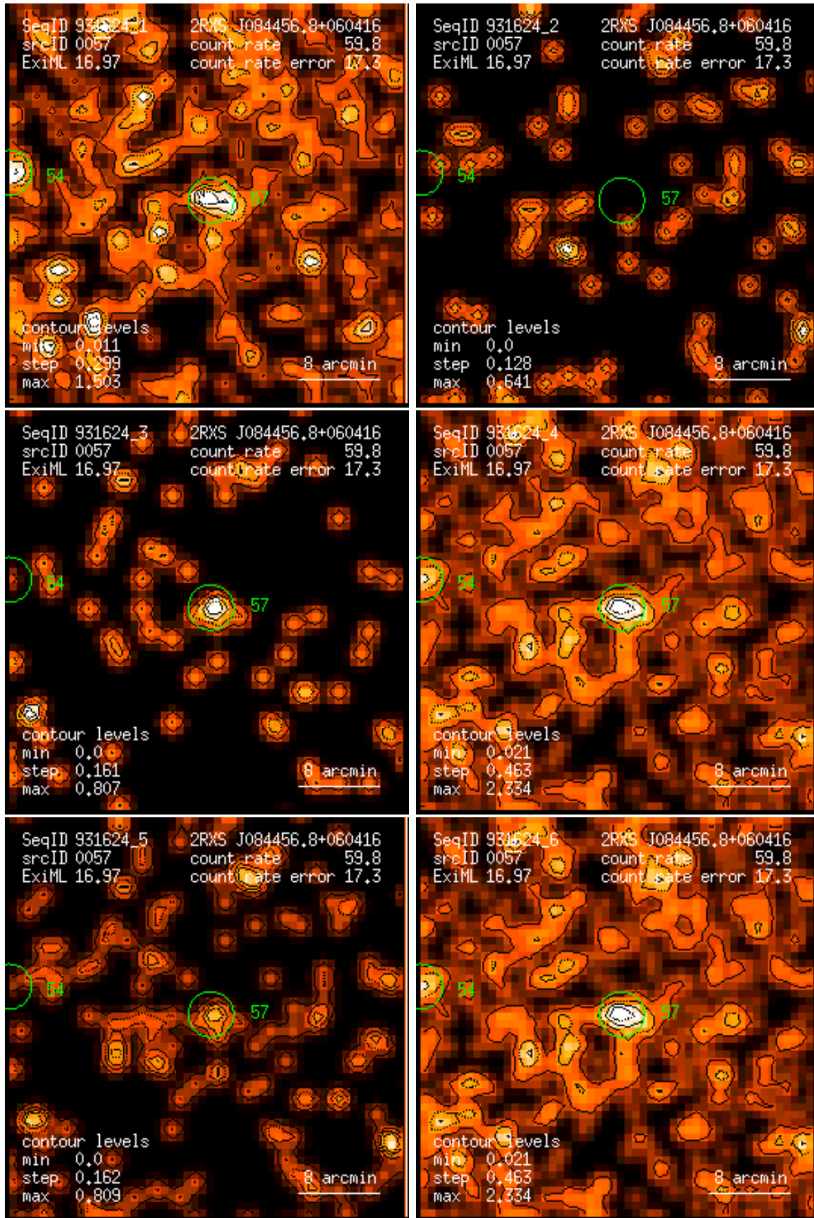
Figure 57: RASS 931624: detection 0057: band rate images, Gaussian filter: (1) PSPC channels 11 – 41, (2) 52 – 90, (3) 91 – 201, (4) 11 – 235, (5) 52 – 201, (6) 11 – 201. Broad band rates in counts/ks. Band rate contour levels in counts/ks/arcmin 2 .
