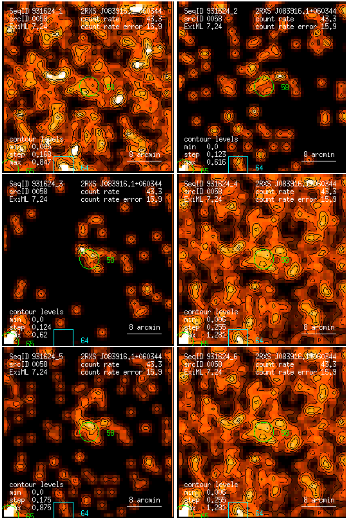
Figure 58: RASS 931624: detection 0058: band rate images, Gaussian filter: (1) PSPC channels 11 – 41, (2) 52 – 90, (3) 91 – 201, (4) 11 – 235, (5) 52 – 201, (6) 11 – 201. Broad band rates in counts/ks. Band rate contour levels in counts/ks/arcmin 2 .
