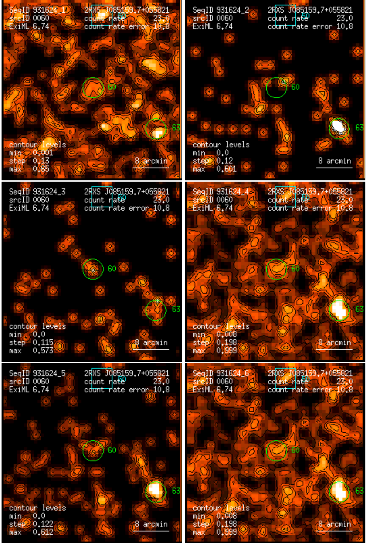
Figure 60: RASS 931624: detection 0060: band rate images, Gaussian filter: (1) PSPC channels 11 – 41, (2) 52 – 90, (3) 91 – 201, (4) 11 – 235, (5) 52 – 201, (6) 11 – 201. Broad band rates in counts/ks. Band rate contour levels in counts/ks/arcmin 2 .
