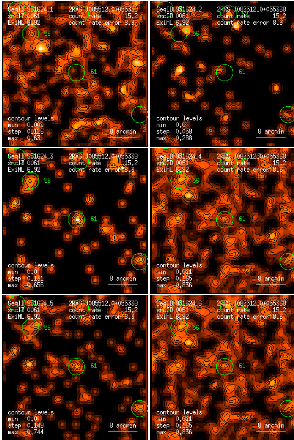
Figure 61: RASS 931624: detection 0061: band rate images, Gaussian filter: (1) PSPC channels 11 – 41, (2) 52 – 90, (3) 91 – 201, (4) 11 – 235, (5) 52 – 201, (6) 11 – 201. Broad band rates in counts/ks. Band rate contour levels in counts/ks/arcmin 2 .
