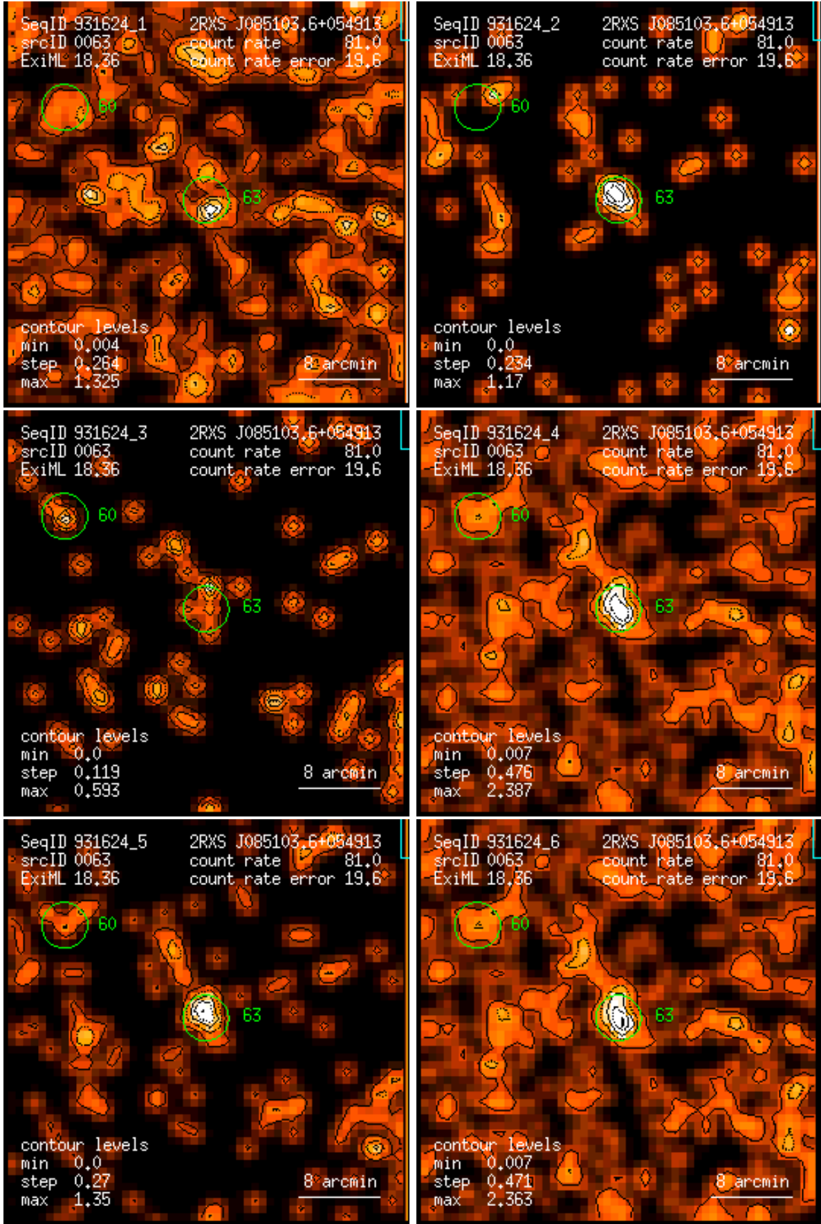
Figure 63: RASS 931624: detection 0063: band rate images, Gaussian filter: (1) PSPC channels 11 – 41, (2) 52 – 90, (3) 91 – 201, (4) 11 – 235, (5) 52 – 201, (6) 11 – 201. Broad band rates in counts/ks. Band rate contour levels in counts/ks/arcmin 2 .
