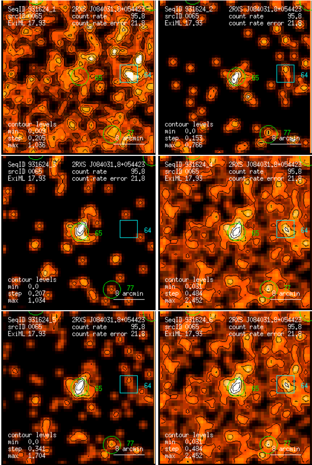
Figure 65: RASS 931624: detection 0065: band rate images, Gaussian filter: (1) PSPC channels 11 – 41, (2) 52 – 90, (3) 91 – 201, (4) 11 – 235, (5) 52 – 201, (6) 11 – 201. Broad band rates in counts/ks. Band rate contour levels in counts/ks/arcmin 2 .
