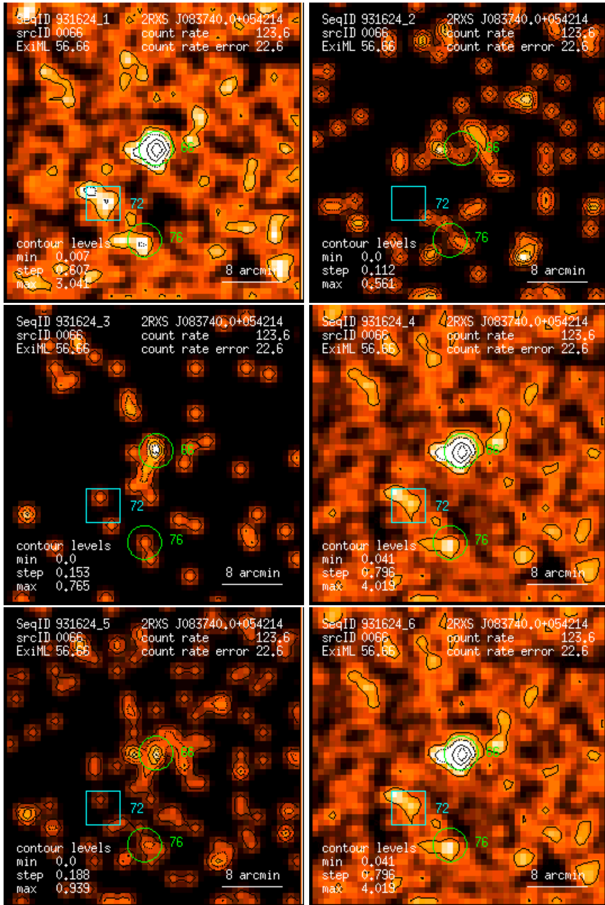
Figure 66: RASS 931624: detection 0066: band rate images, Gaussian filter: (1) PSPC channels 11 – 41, (2) 52 – 90, (3) 91 – 201, (4) 11 – 235, (5) 52 – 201, (6) 11 – 201. Broad band rates in counts/ks. Band rate contour levels in counts/ks/arcmin 2 .
