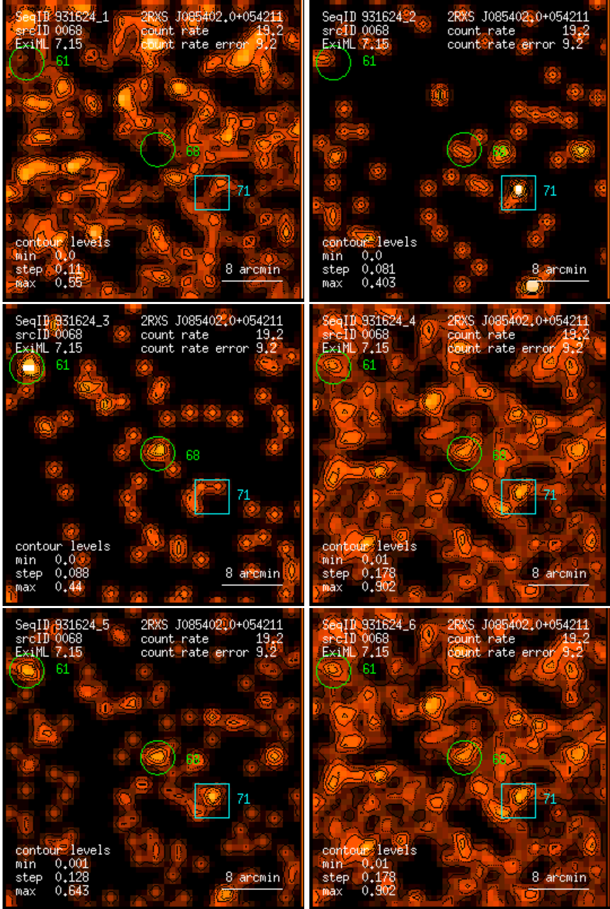
Figure 68: RASS 931624: detection 0068: band rate images, Gaussian filter: (1) PSPC channels 11 – 41, (2) 52 – 90, (3) 91 – 201, (4) 11 – 235, (5) 52 – 201, (6) 11 – 201. Broad band rates in counts/ks. Band rate contour levels in counts/ks/arcmin 2 .
