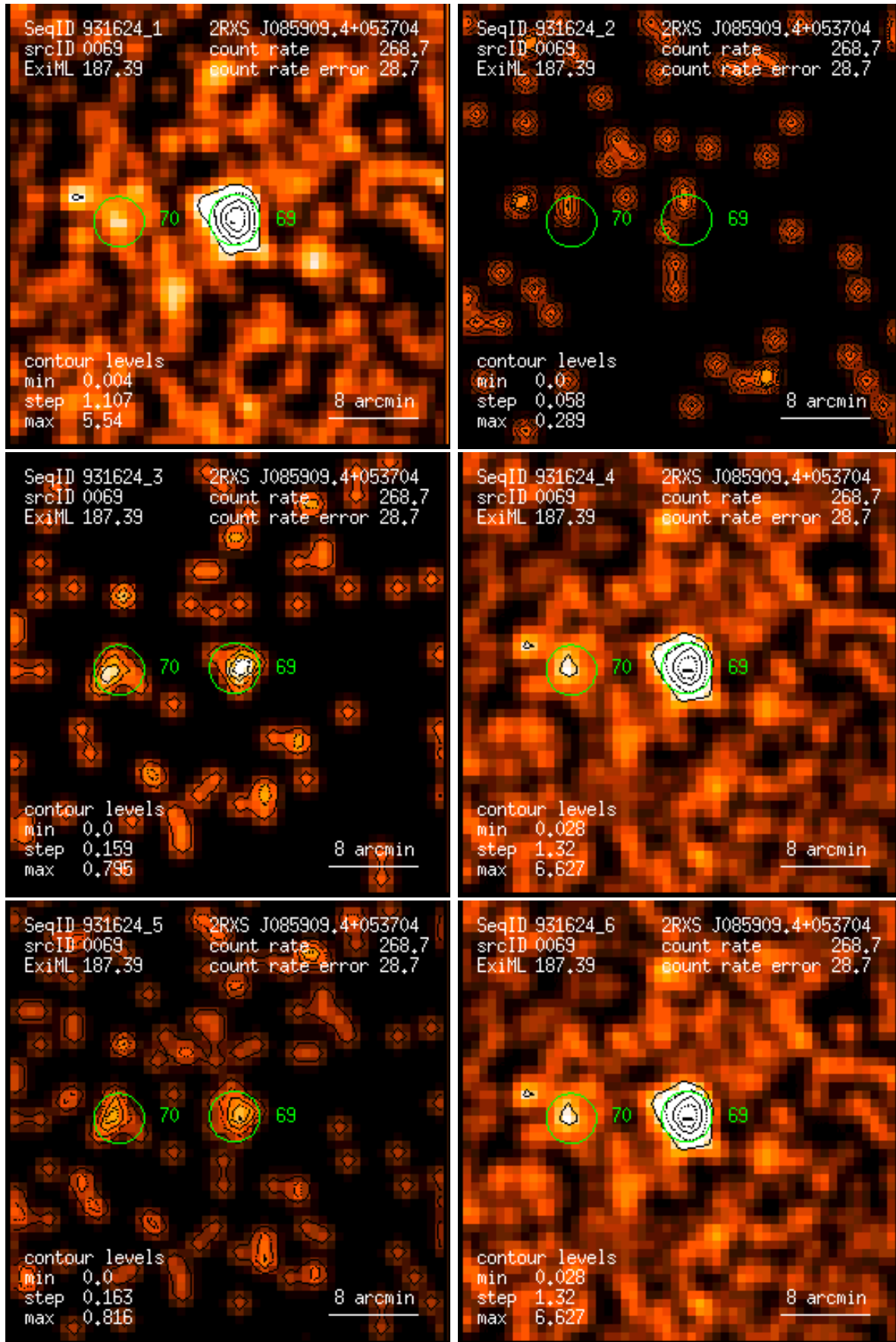
Figure 69: RASS 931624: detection 0069: band rate images, Gaussian filter: (1) PSPC channels 11 – 41, (2) 52 – 90, (3) 91 – 201, (4) 11 – 235, (5) 52 – 201, (6) 11 – 201. Broad band rates in counts/ks. Band rate contour levels in counts/ks/arcmin 2 .
