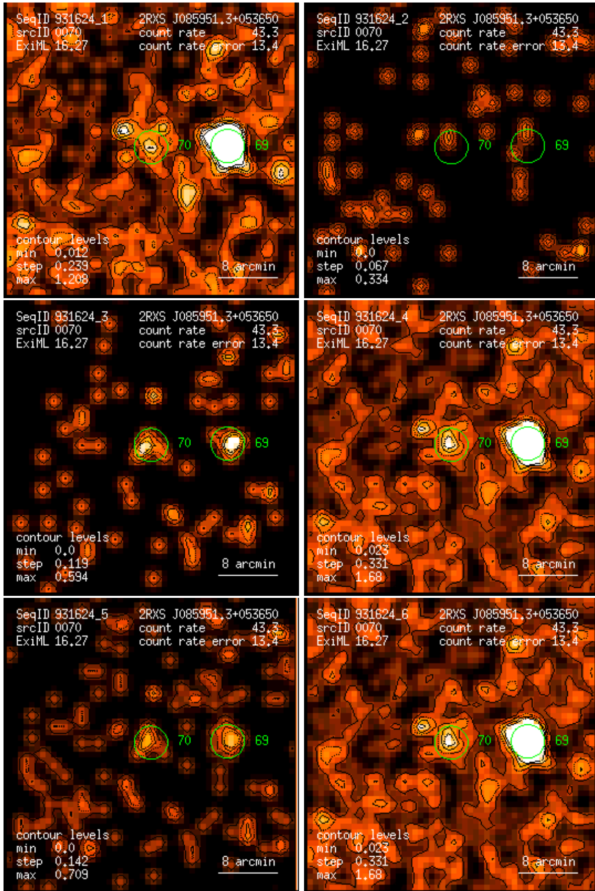
Figure 70: RASS 931624: detection 0070: band rate images, Gaussian filter: (1) PSPC channels 11 – 41, (2) 52 – 90, (3) 91 – 201, (4) 11 – 235, (5) 52 – 201, (6) 11 – 201. Broad band rates in counts/ks. Band rate contour levels in counts/ks/arcmin 2 .
