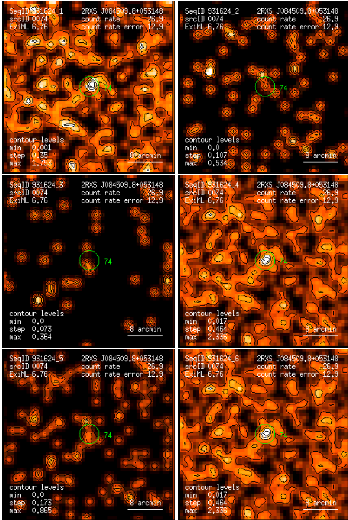
Figure 74: RASS 931624: detection 0074: band rate images, Gaussian filter: (1) PSPC channels 11 – 41, (2) 52 – 90, (3) 91 – 201, (4) 11 – 235, (5) 52 – 201, (6) 11 – 201. Broad band rates in counts/ks. Band rate contour levels in counts/ks/arcmin 2 .
