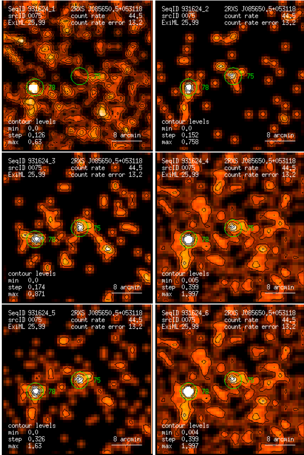
Figure 75: RASS 931624: detection 0075: band rate images, Gaussian filter: (1) PSPC channels 11 – 41, (2) 52 – 90, (3) 91 – 201, (4) 11 – 235, (5) 52 – 201, (6) 11 – 201. Broad band rates in counts/ks. Band rate contour levels in counts/ks/arcmin 2 .
