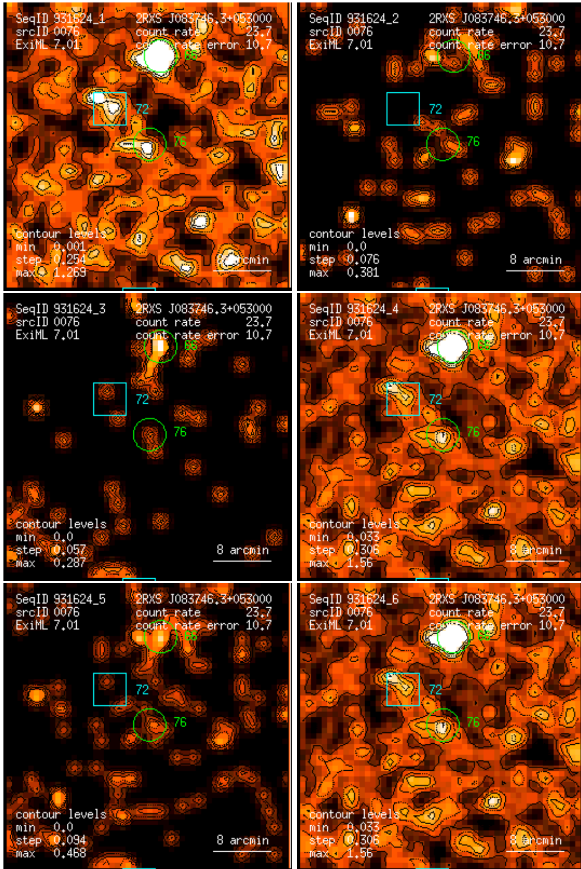
Figure 76: RASS 931624: detection 0076: band rate images, Gaussian filter: (1) PSPC channels 11 – 41, (2) 52 – 90, (3) 91 – 201, (4) 11 – 235, (5) 52 – 201, (6) 11 – 201. Broad band rates in counts/ks. Band rate contour levels in counts/ks/arcmin 2 .
