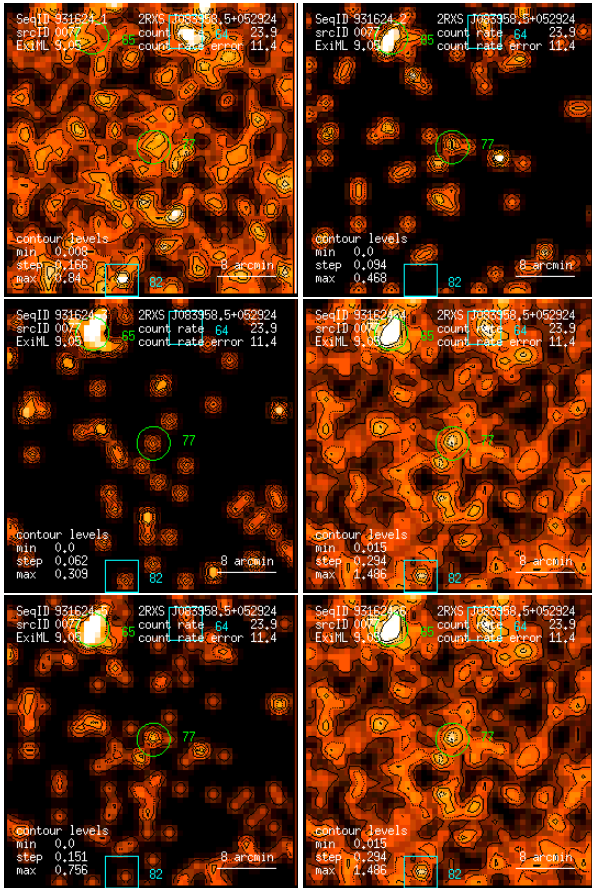
Figure 77: RASS 931624: detection 0077: band rate images, Gaussian filter: (1) PSPC channels 11 – 41, (2) 52 – 90, (3) 91 – 201, (4) 11 – 235, (5) 52 – 201, (6) 11 – 201. Broad band rates in counts/ks. Band rate contour levels in counts/ks/arcmin 2 .
