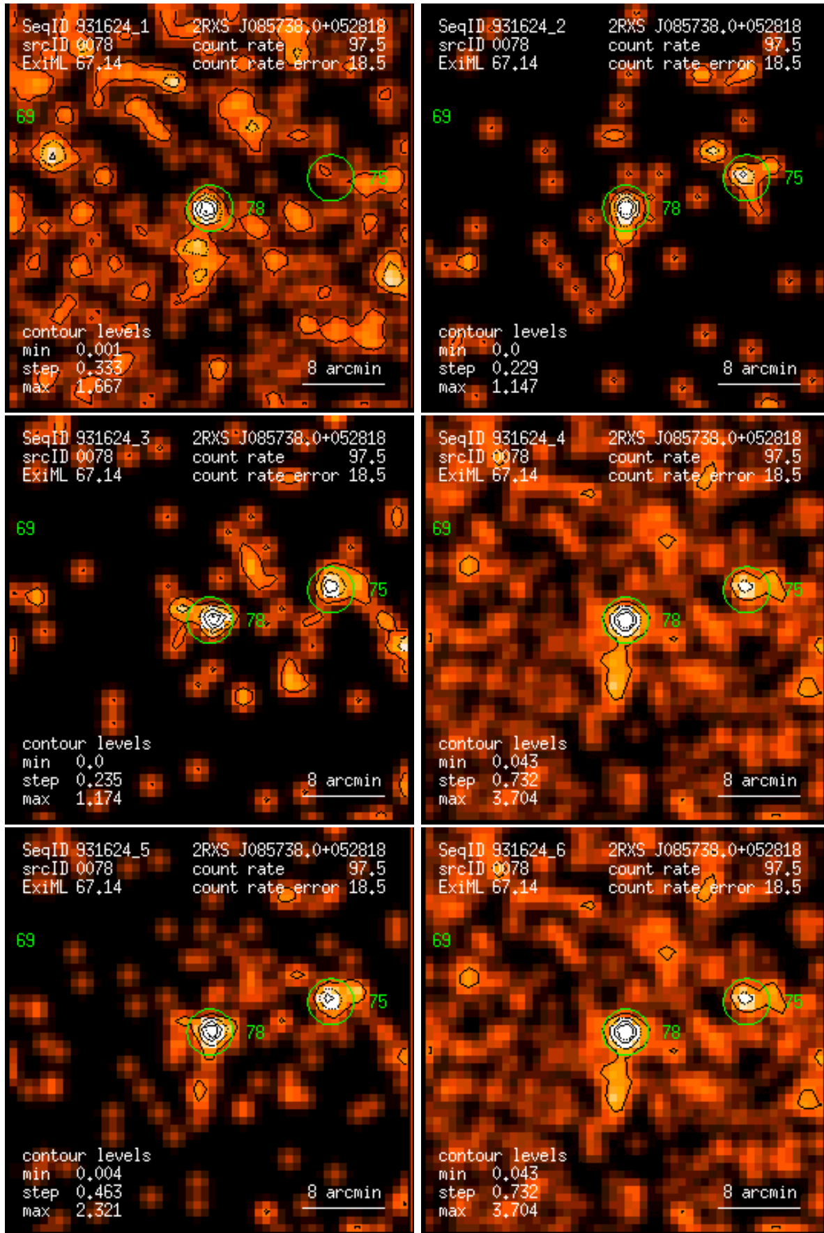
Figure 78: RASS 931624: detection 0078: band rate images, Gaussian filter: (1) PSPC channels 11 – 41, (2) 52 – 90, (3) 91 – 201, (4) 11 – 235, (5) 52 – 201, (6) 11 – 201. Broad band rates in counts/ks. Band rate contour levels in counts/ks/arcmin 2 .
