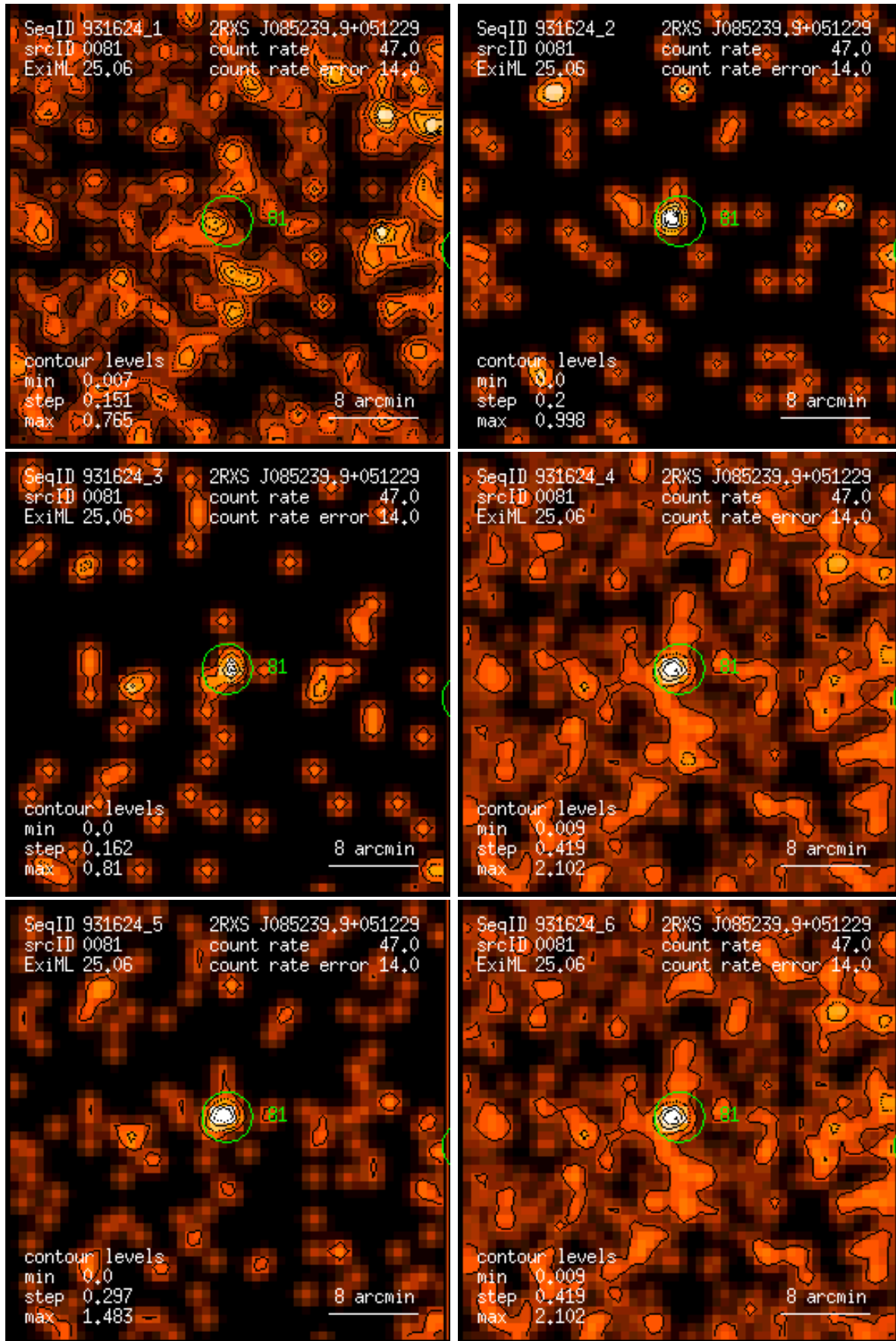
Figure 81: RASS 931624: detection 0081: band rate images, Gaussian filter: (1) PSPC channels 11 – 41, (2) 52 – 90, (3) 91 – 201, (4) 11 – 235, (5) 52 – 201, (6) 11 – 201. Broad band rates in counts/ks. Band rate contour levels in counts/ks/arcmin 2 .
