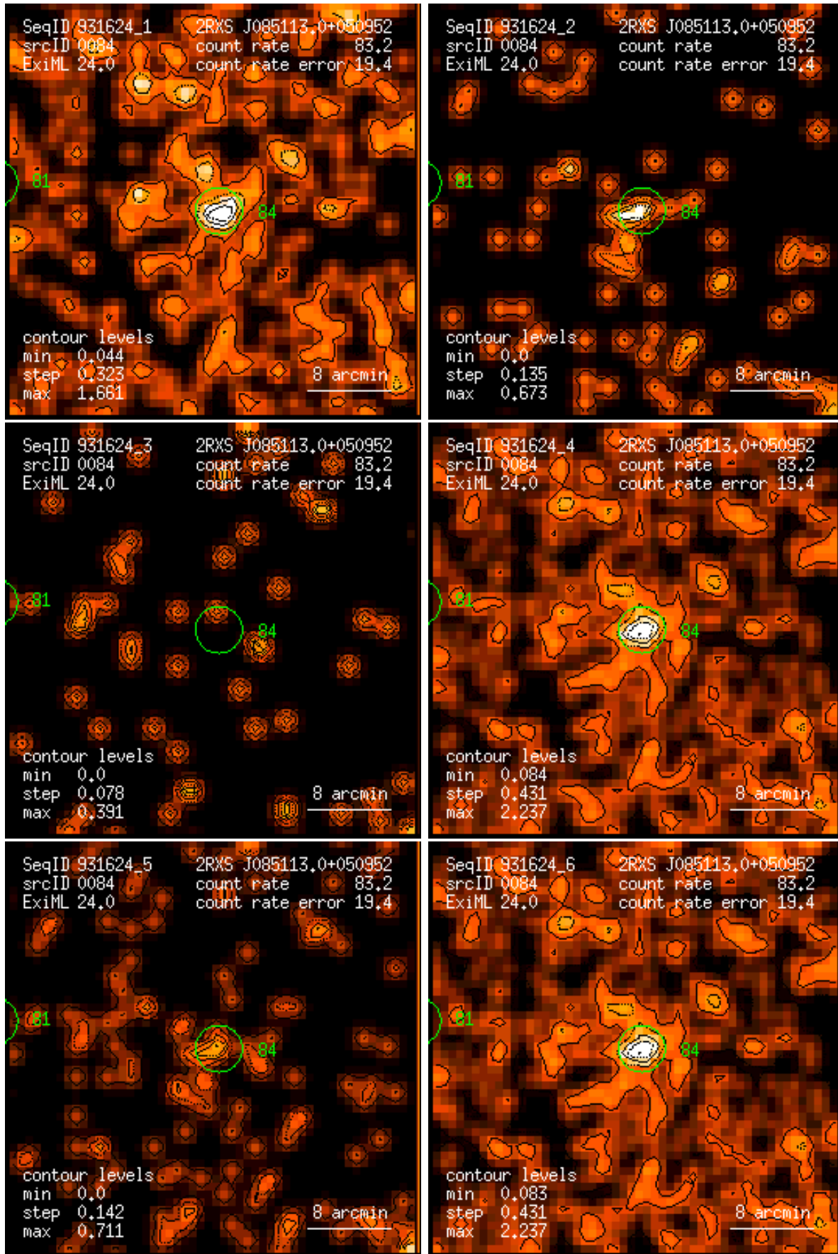
Figure 84: RASS 931624: detection 0084: band rate images, Gaussian filter: (1) PSPC channels 11 – 41, (2) 52 – 90, (3) 91 – 201, (4) 11 – 235, (5) 52 – 201, (6) 11 – 201. Broad band rates in counts/ks. Band rate contour levels in counts/ks/arcmin 2 .
