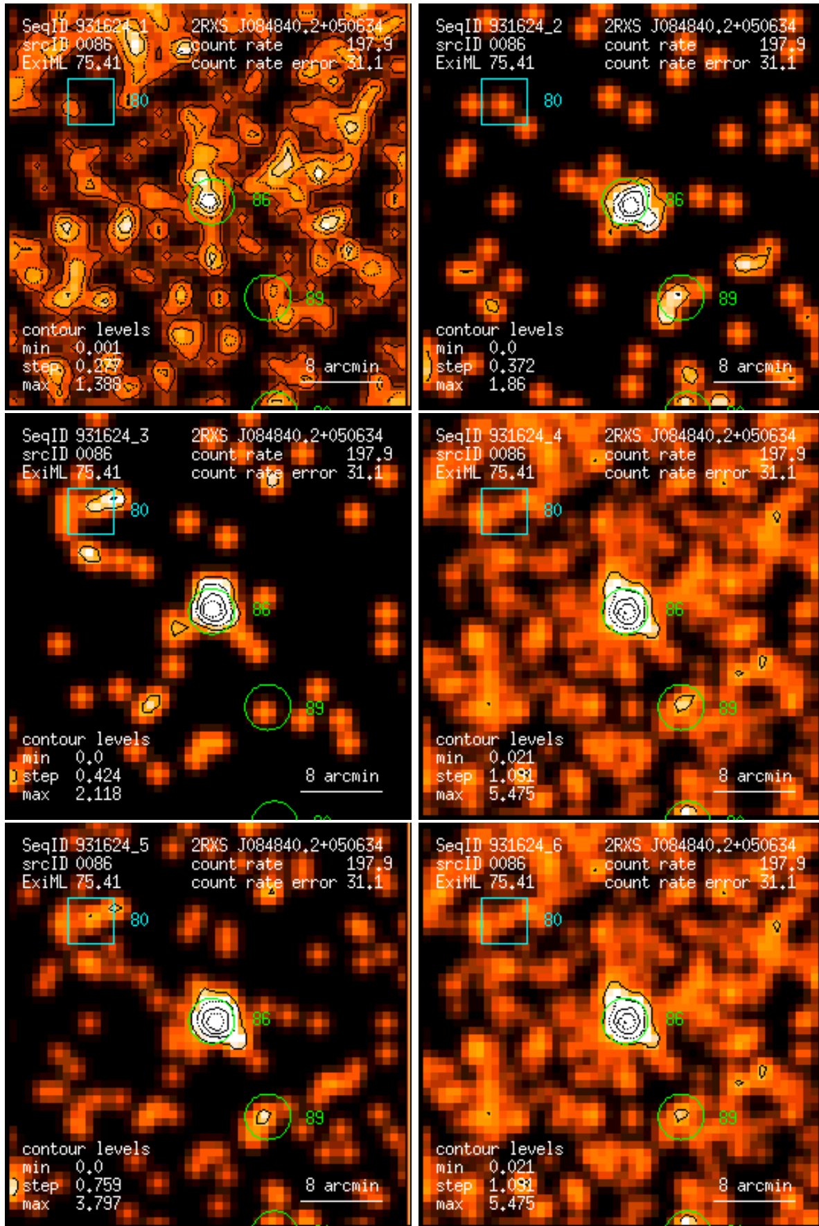
Figure 86: RASS 931624: detection 0086: band rate images, Gaussian filter: (1) PSPC channels 11 – 41, (2) 52 – 90, (3) 91 – 201, (4) 11 – 235, (5) 52 – 201, (6) 11 – 201. Broad band rates in counts/ks. Band rate contour levels in counts/ks/arcmin 2 .
