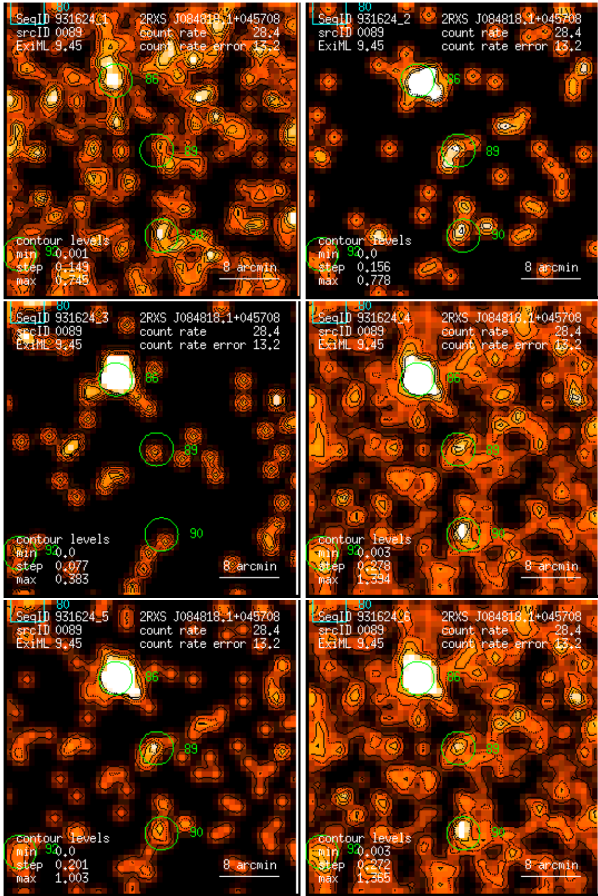
Figure 89: RASS 931624: detection 0089: band rate images, Gaussian filter: (1) PSPC channels 11 – 41, (2) 52 – 90, (3) 91 – 201, (4) 11 – 235, (5) 52 – 201, (6) 11 – 201. Broad band rates in counts/ks. Band rate contour levels in counts/ks/arcmin 2 .
