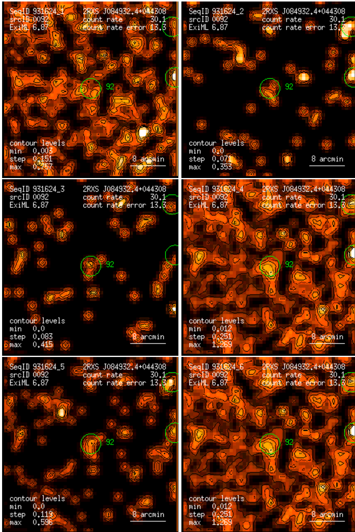
Figure 92: RASS 931624: detection 0092: band rate images, Gaussian filter: (1) PSPC channels 11 – 41, (2) 52 – 90, (3) 91 – 201, (4) 11 – 235, (5) 52 – 201, (6) 11 – 201. Broad band rates in counts/ks. Band rate contour levels in counts/ks/arcmin 2 .
