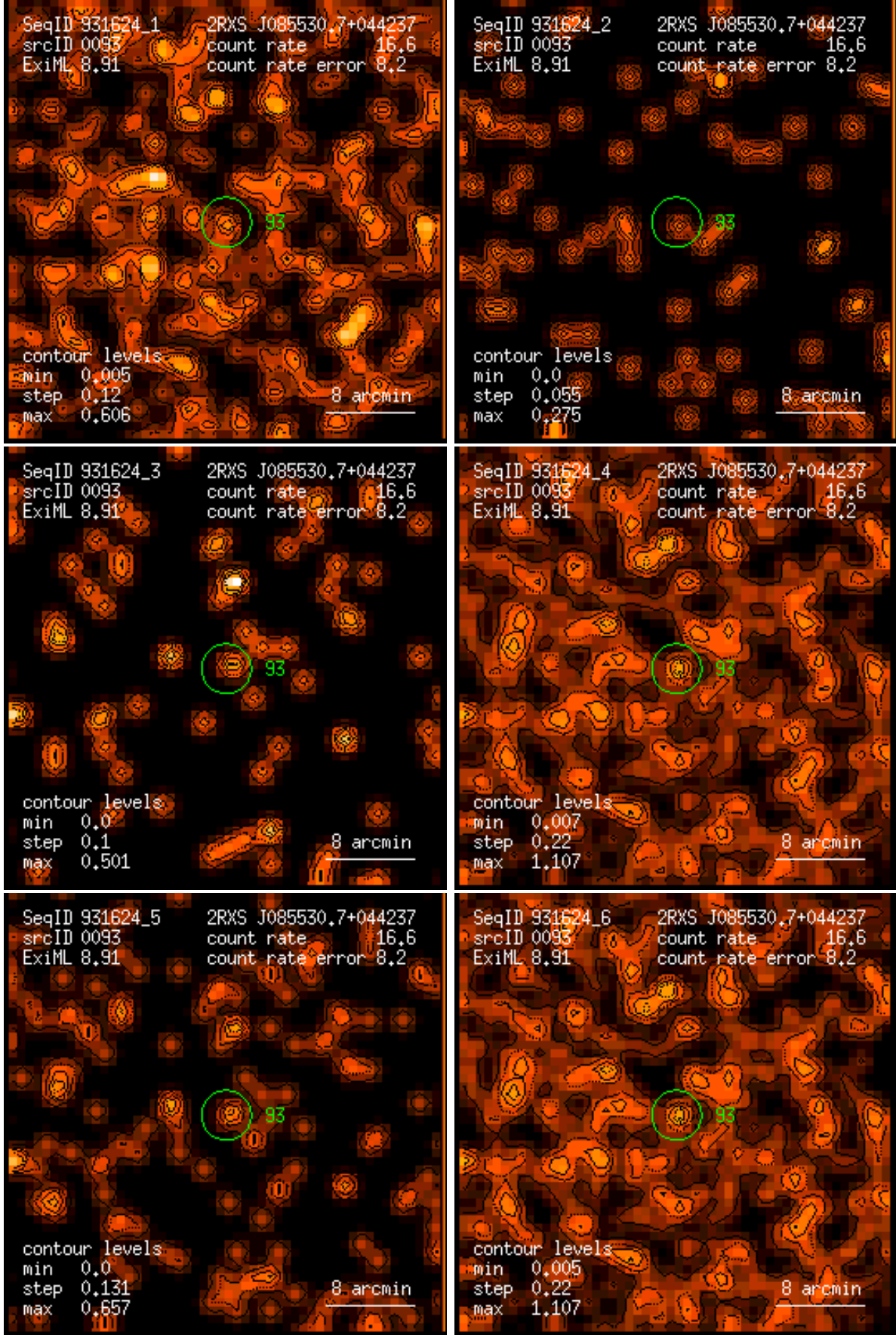
Figure 93: RASS 931624: detection 0093: band rate images, Gaussian filter: (1) PSPC channels 11 – 41, (2) 52 – 90, (3) 91 – 201, (4) 11 – 235, (5) 52 – 201, (6) 11 – 201. Broad band rates in counts/ks. Band rate contour levels in counts/ks/arcmin 2 .
