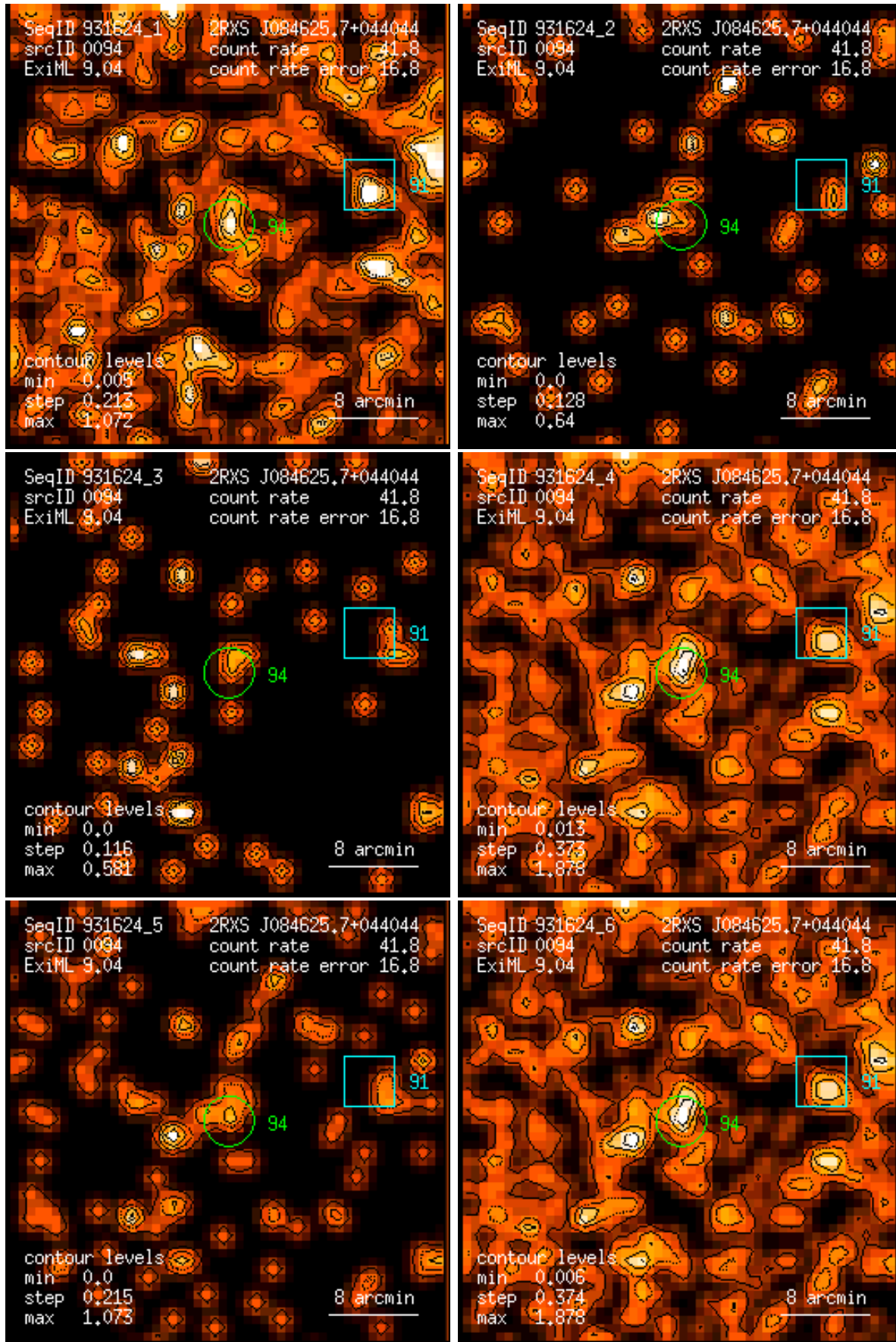
Figure 94: RASS 931624: detection 0094: band rate images, Gaussian filter: (1) PSPC channels 11 – 41, (2) 52 – 90, (3) 91 – 201, (4) 11 – 235, (5) 52 – 201, (6) 11 – 201. Broad band rates in counts/ks. Band rate contour levels in counts/ks/arcmin 2 .
