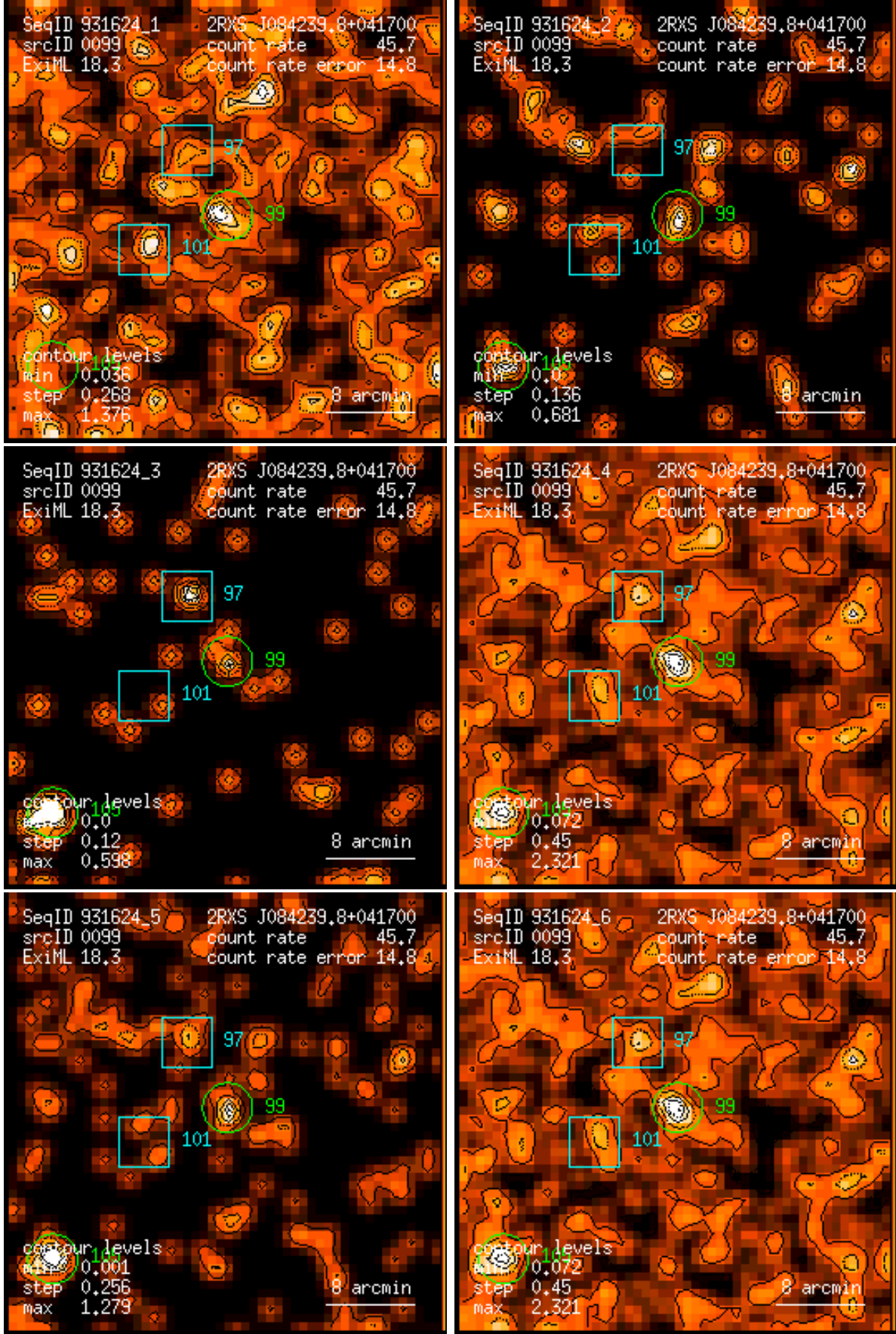
Figure 99: RASS 931624: detection 0099: band rate images, Gaussian filter: (1) PSPC channels 11 – 41, (2) 52 – 90, (3) 91 – 201, (4) 11 – 235, (5) 52 – 201, (6) 11 – 201. Broad band rates in counts/ks. Band rate contour levels in counts/ks/arcmin 2 .
