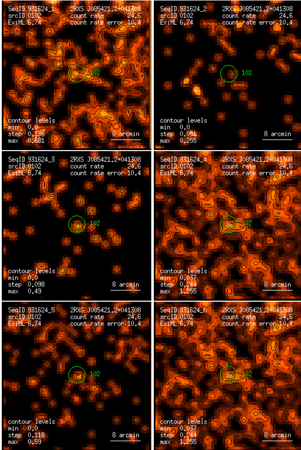
Figure 102: RASS 931624: detection 0102: band rate images, Gaussian filter: (1) PSPC channels 11 – 41, (2) 52 – 90, (3) 91 – 201, (4) 11 – 235, (5) 52 – 201, (6) 11 – 201. Broad band rates in counts/ks. Band rate contour levels in counts/ks/arcmin 2 .
