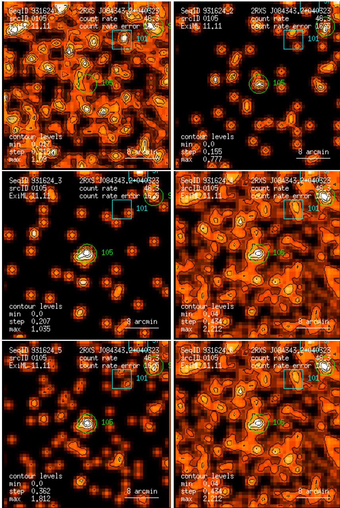
Figure 105: RASS 931624: detection 0105: band rate images, Gaussian filter: (1) PSPC channels 11 – 41, (2) 52 – 90, (3) 91 – 201, (4) 11 – 235, (5) 52 – 201, (6) 11 – 201. Broad band rates in counts/ks. Band rate contour levels in counts/ks/arcmin 2 .
