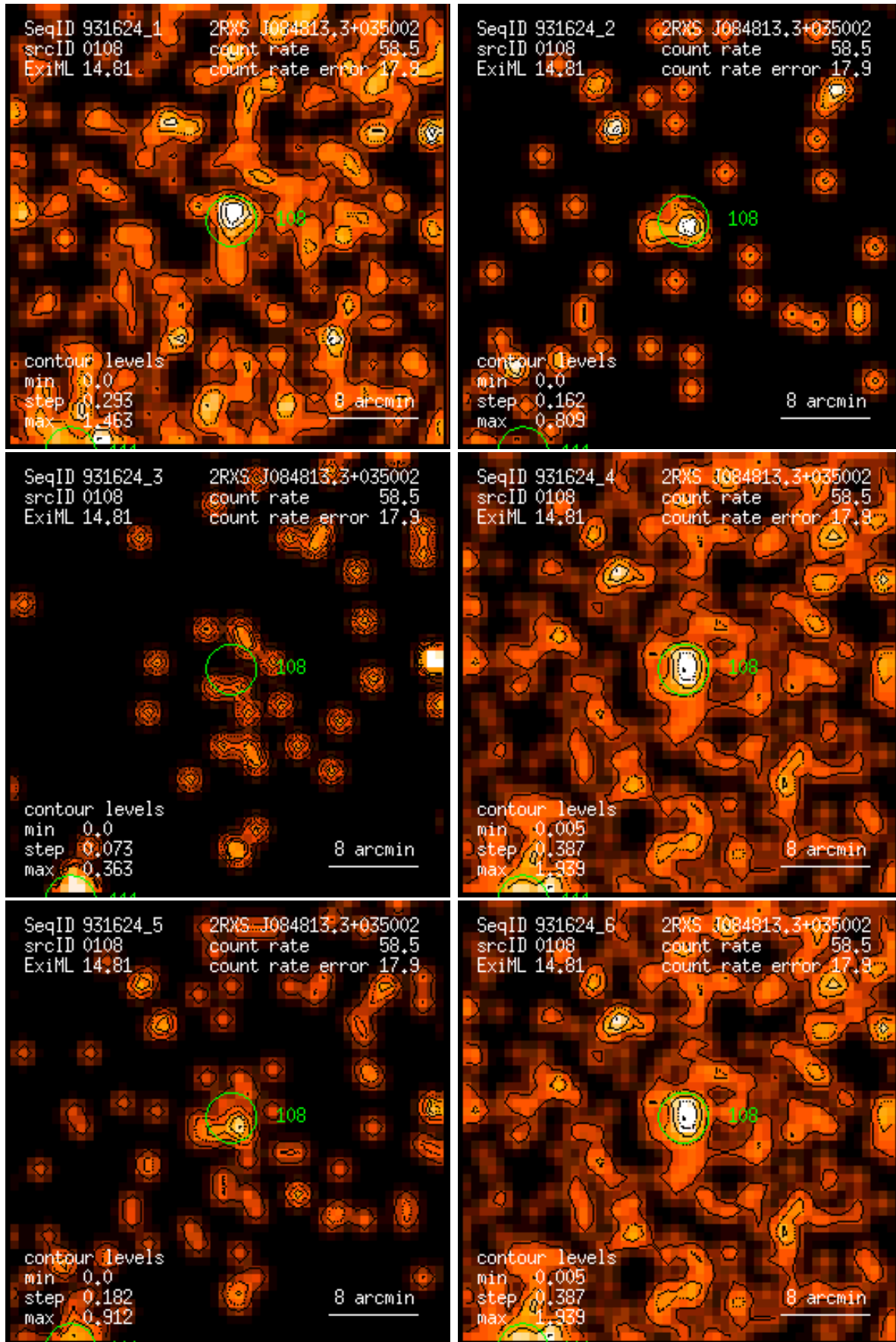
Figure 108: RASS 931624: detection 0108: band rate images, Gaussian filter: (1) PSPC channels 11 – 41, (2) 52 – 90, (3) 91 – 201, (4) 11 – 235, (5) 52 – 201, (6) 11 – 201. Broad band rates in counts/ks. Band rate contour levels in counts/ks/arcmin 2 .
