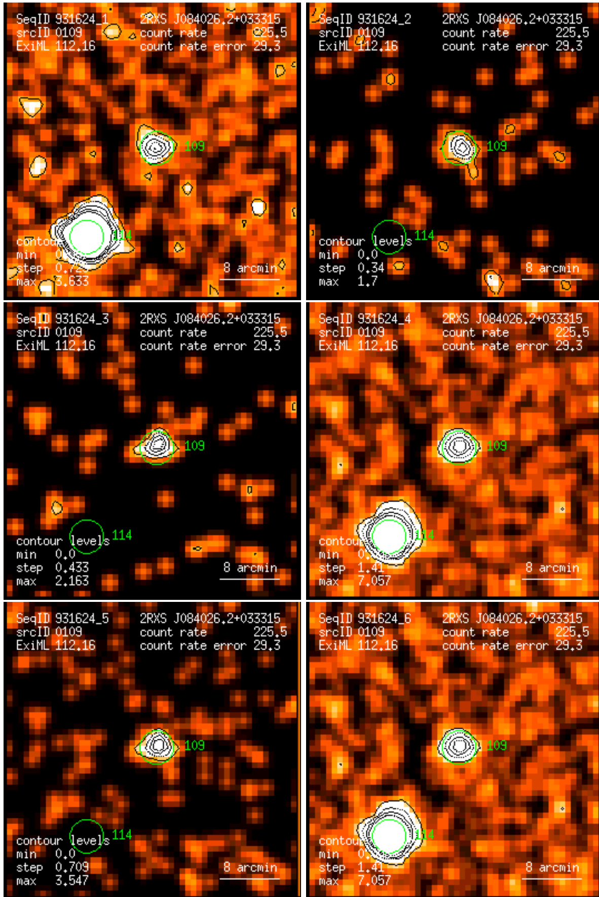
Figure 109: RASS 931624: detection 0109: band rate images, Gaussian filter: (1) PSPC channels 11 – 41, (2) 52 – 90, (3) 91 – 201, (4) 11 – 235, (5) 52 – 201, (6) 11 – 201. Broad band rates in counts/ks. Band rate contour levels in counts/ks/arcmin 2 .
