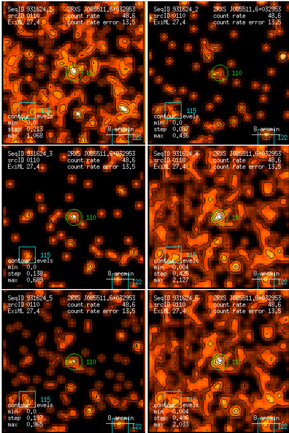
Figure 110: RASS 931624: detection 0110: band rate images, Gaussian filter: (1) PSPC channels 11 – 41, (2) 52 – 90, (3) 91 – 201, (4) 11 – 235, (5) 52 – 201, (6) 11 – 201. Broad band rates in counts/ks. Band rate contour levels in counts/ks/arcmin 2 .
